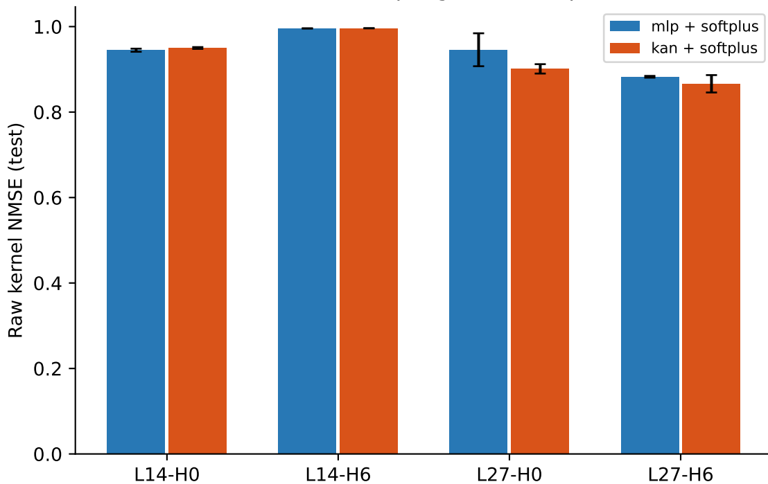
Importance sampling, 10,000 steps
