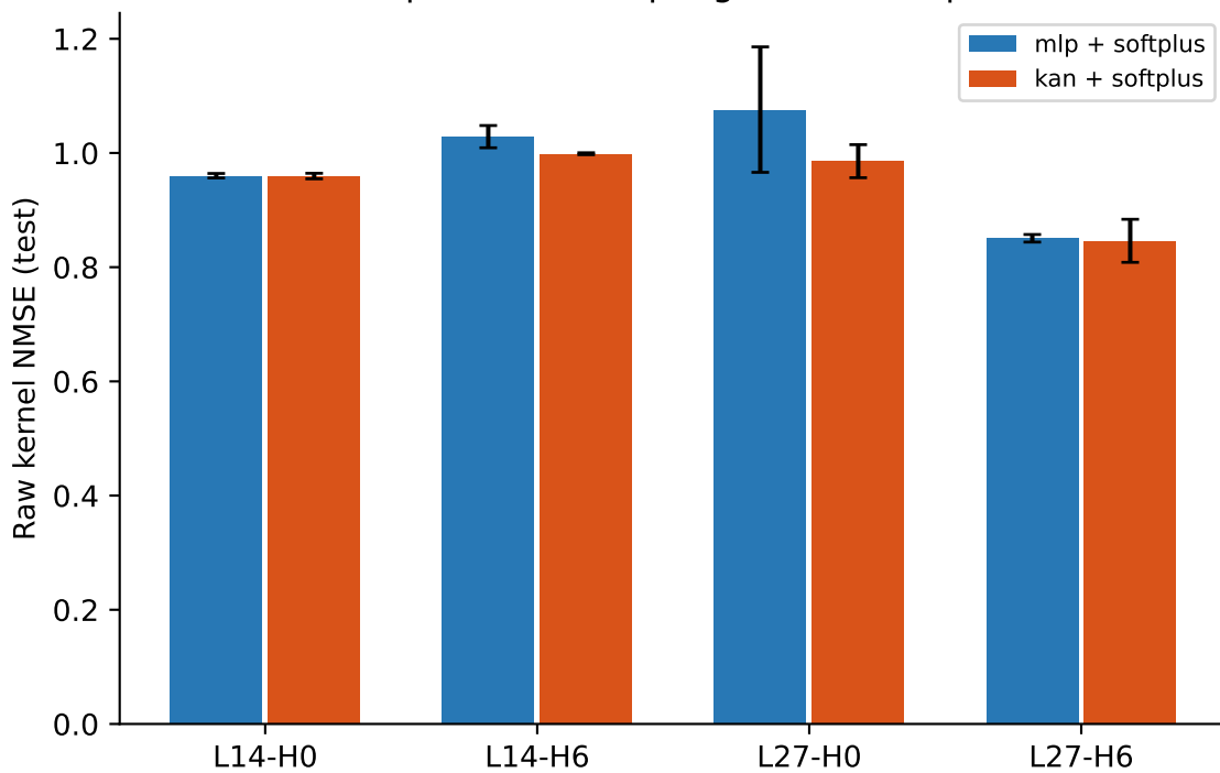
Importance sampling, 10,000 steps
