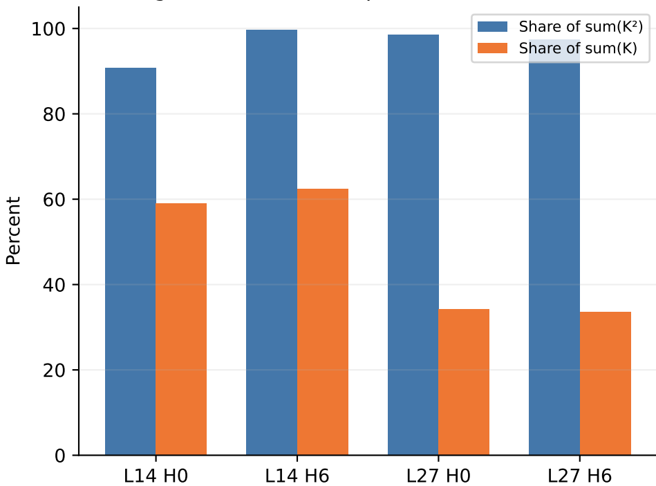
Largest \sim 0.1\% kernel pairs (256 documents)
