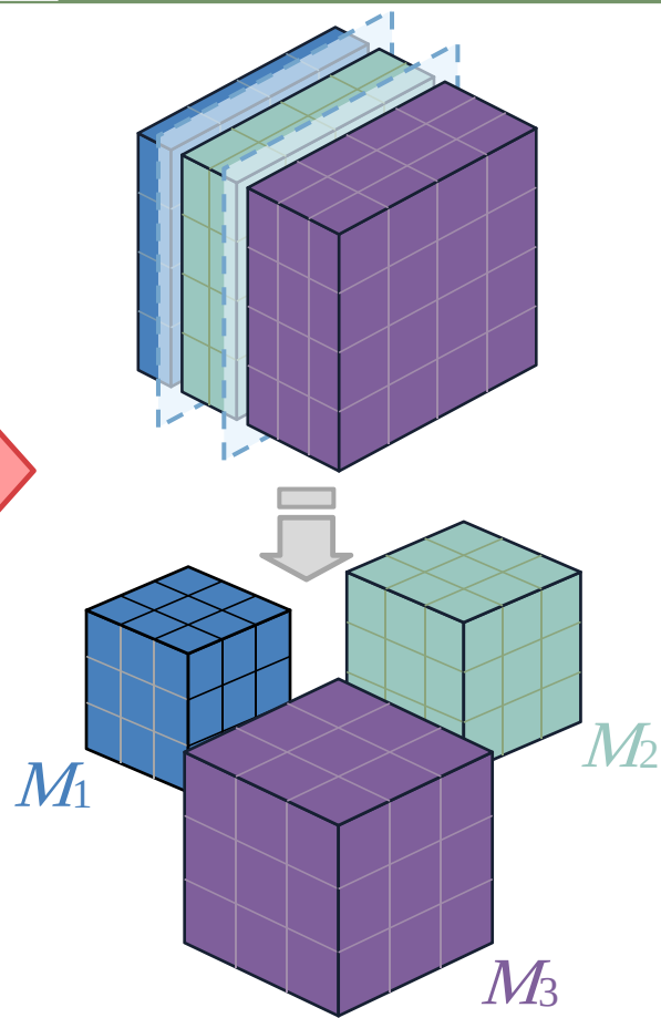
Model Slicing
