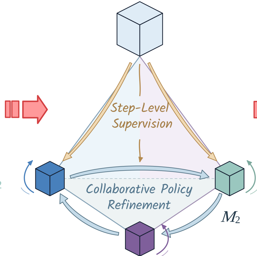
Pyramid Learning
