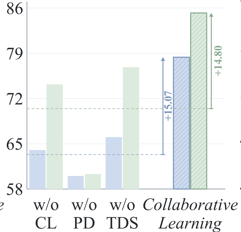
MATH
