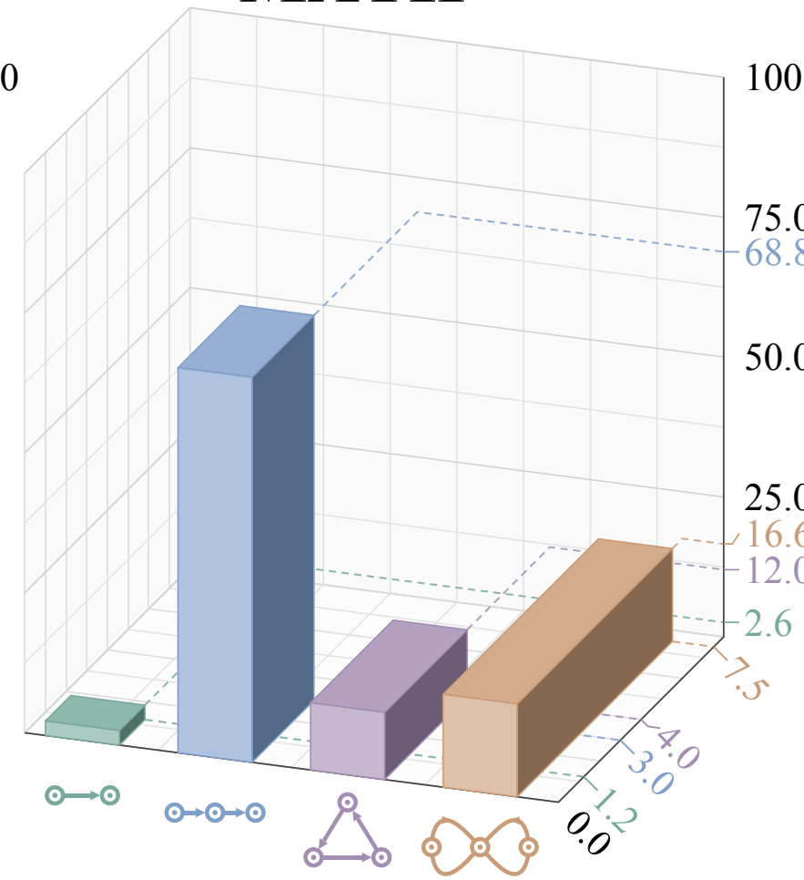
MATH
