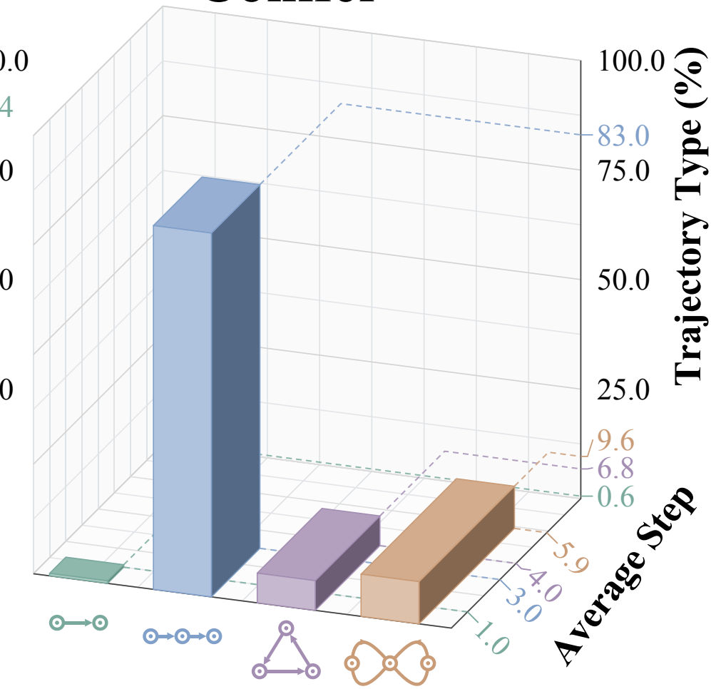
Conifer
