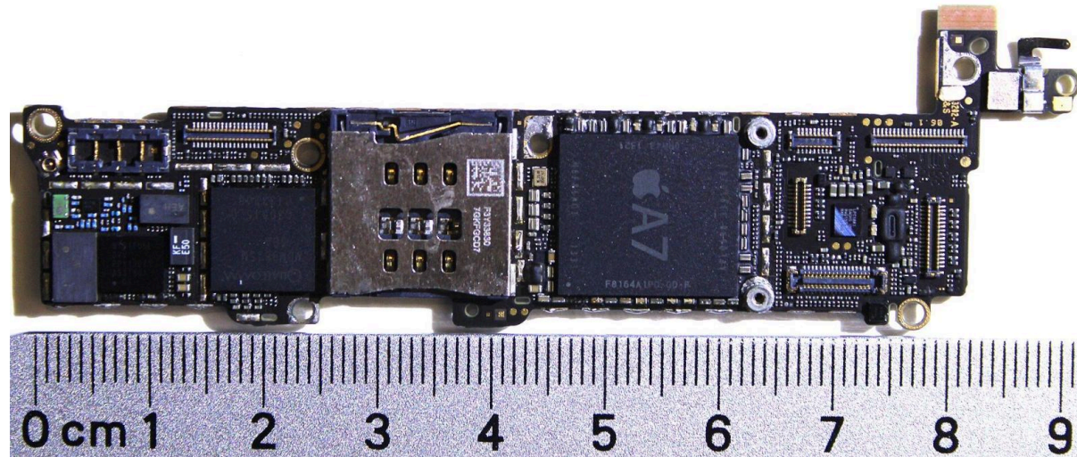
Sonic8400, iPhone 5s logic board with A7 , 2020 · Wikimedia Commons, CC BY-SA 4.0.
