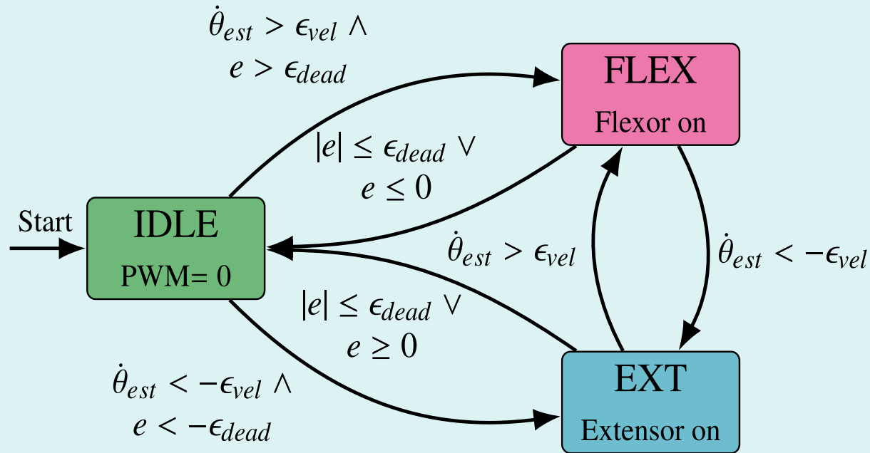
Supervisory flowchart
