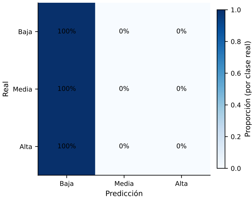
Confusion matrix (row-normalized)
