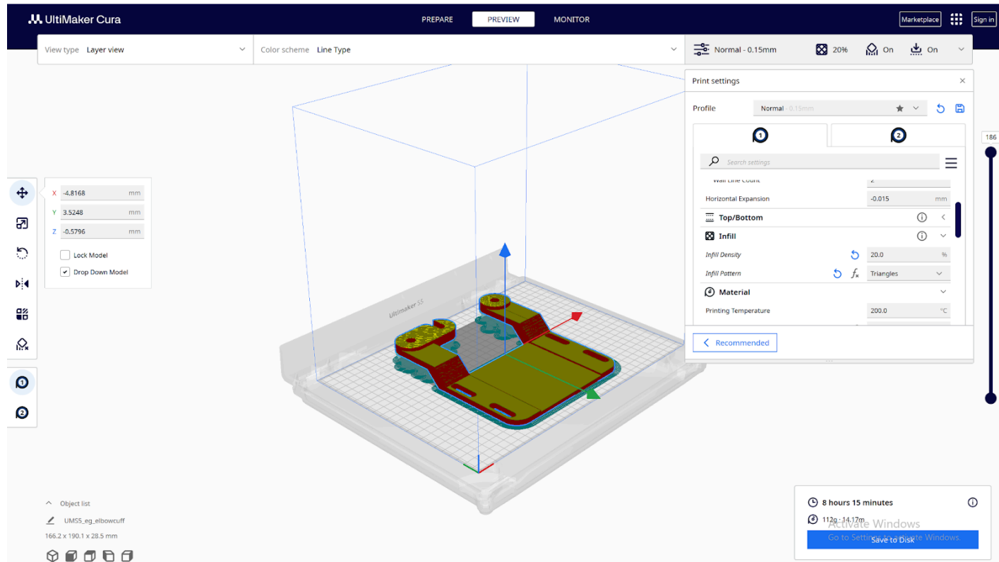
Forearm/Elbow-Cuff Material: PLA
