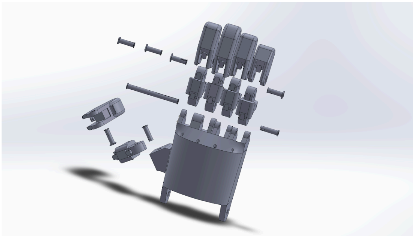
Exploded View
