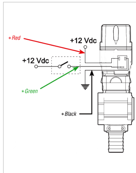
3-wire valve
