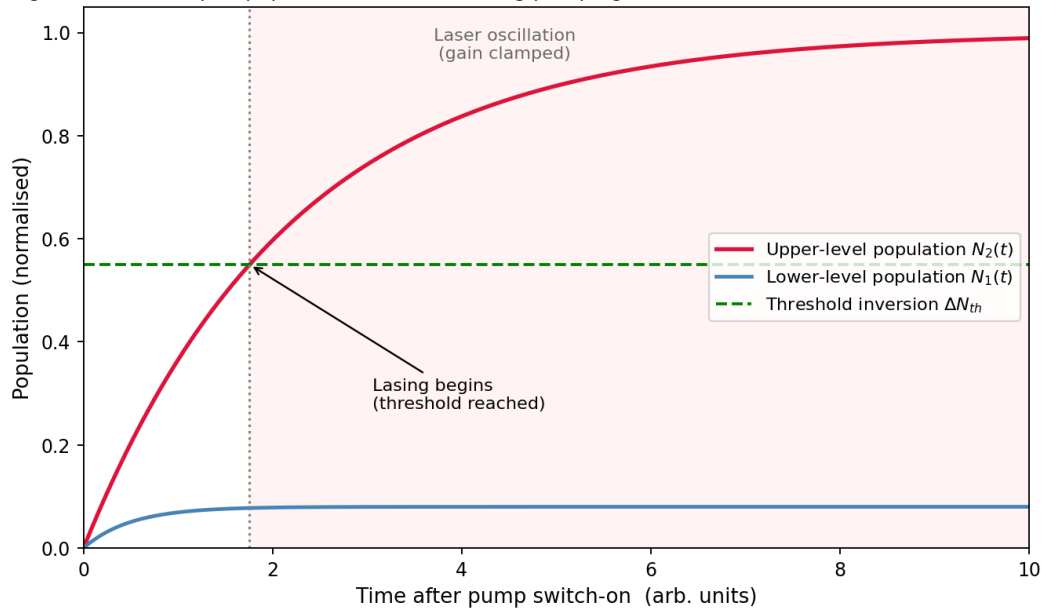
Fig. 1.12D Build-up of population inversion during pumping, and the onset of laser oscillation at threshold
