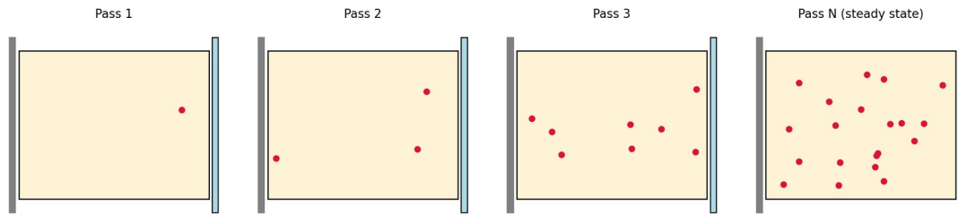
Fig. 1.4A Photon avalanche: successive resonator round trips multiply the number of coherent, stimulated-emission photons until the beam reaches its steady-state (saturated) intensity.
