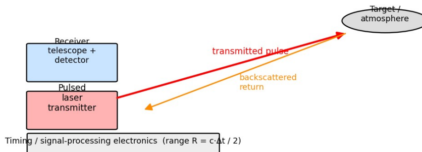
Fig. 5.2 Principle of LIDAR: a pulsed laser transmitter and a co-located receiver telescope/detector determine target range from the round-trip time of flight of the backscattered pulse.
