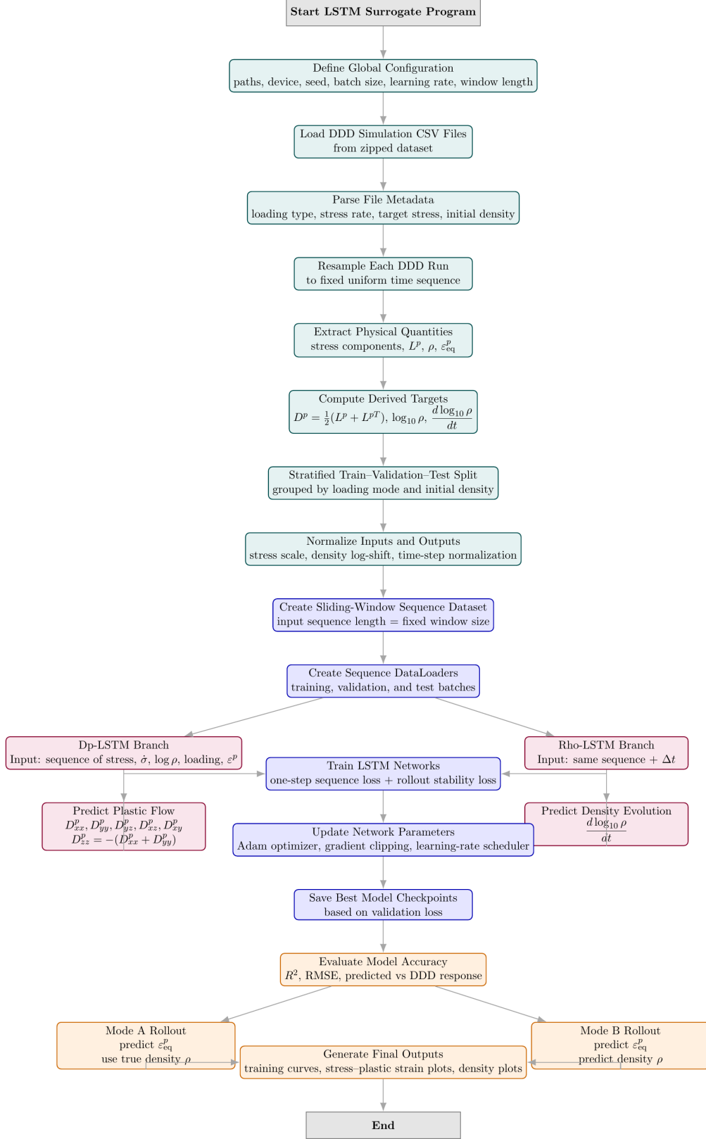
Figure 2: Flowchart of the LSTM-based surrogate modelling pipeline for DDD data
