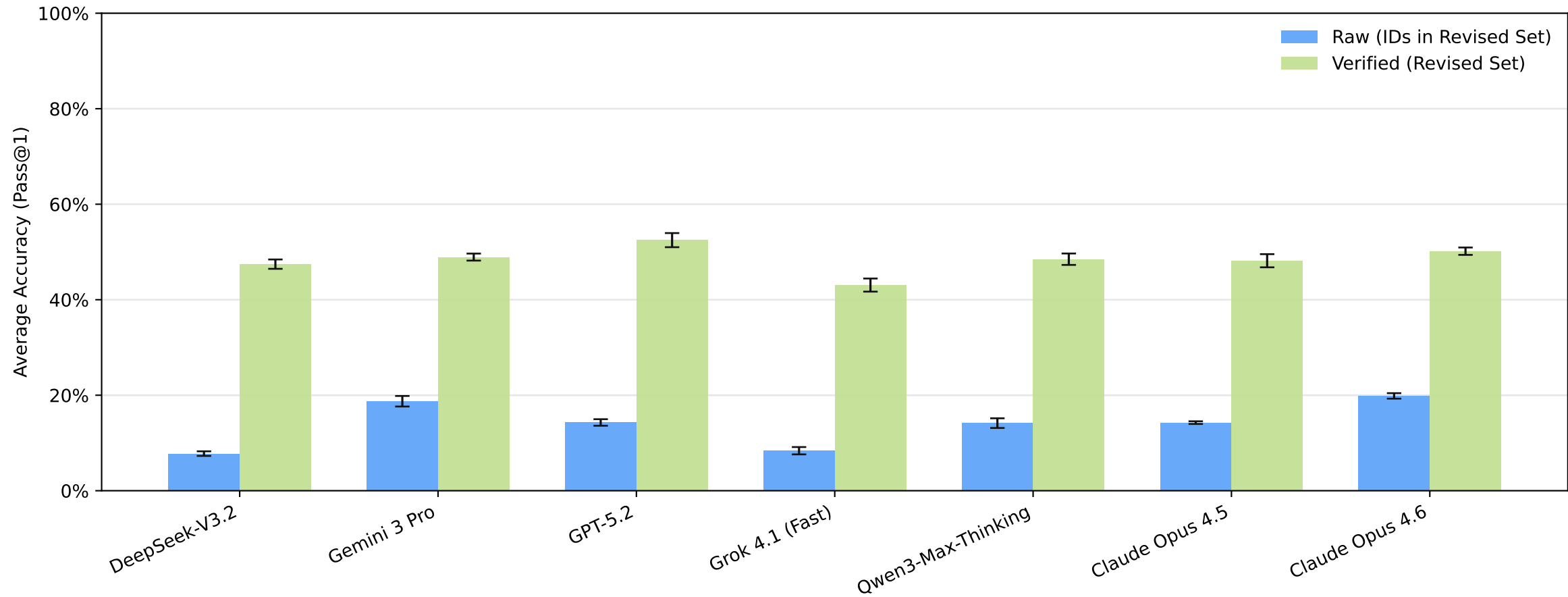
HLE-Raw vs HLE-Verified on Revised Set
