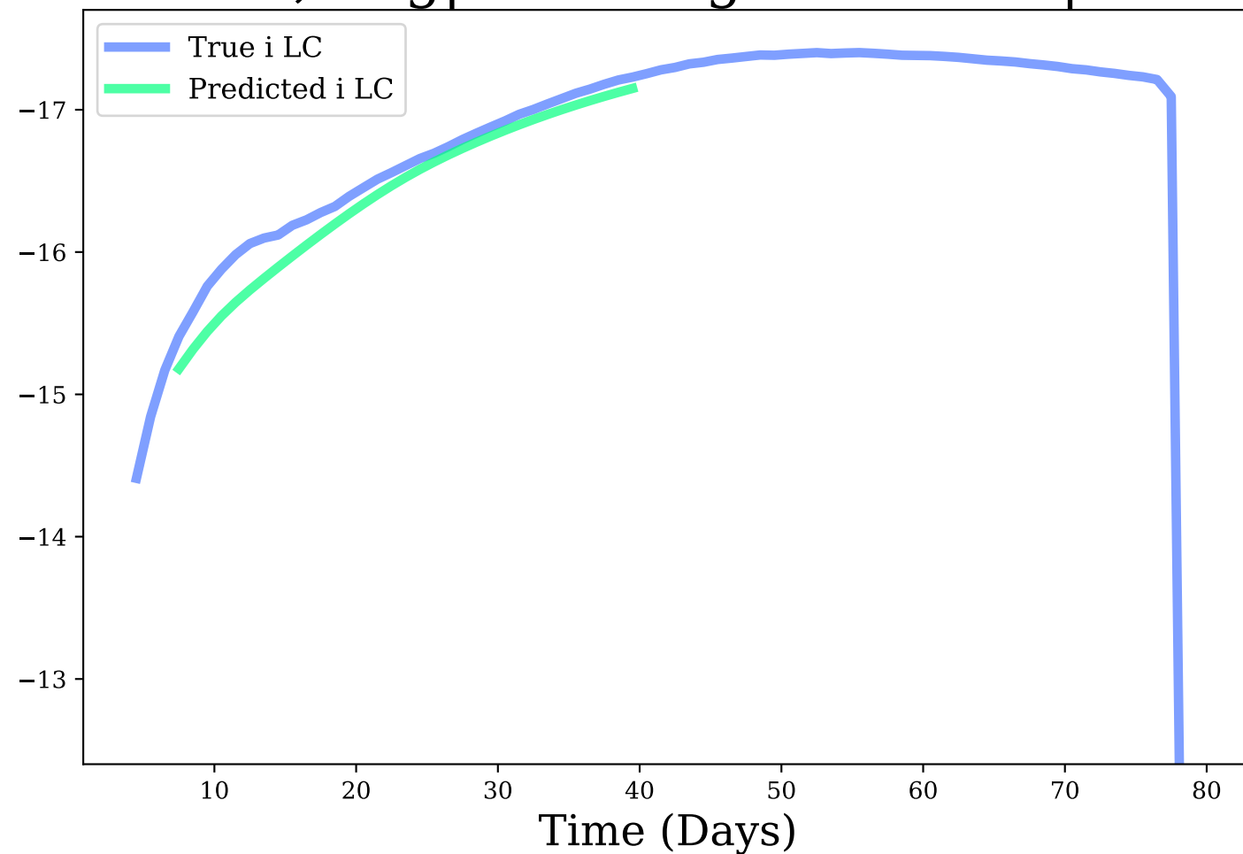
i-band, Avg|Max Mag Diff: 0.14 | 0.33
