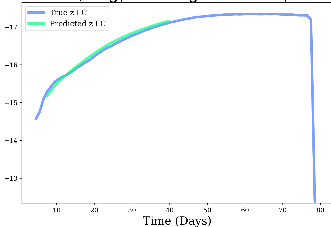
z-band, Avg|Max Mag Diff: 0.07 | 0.12
