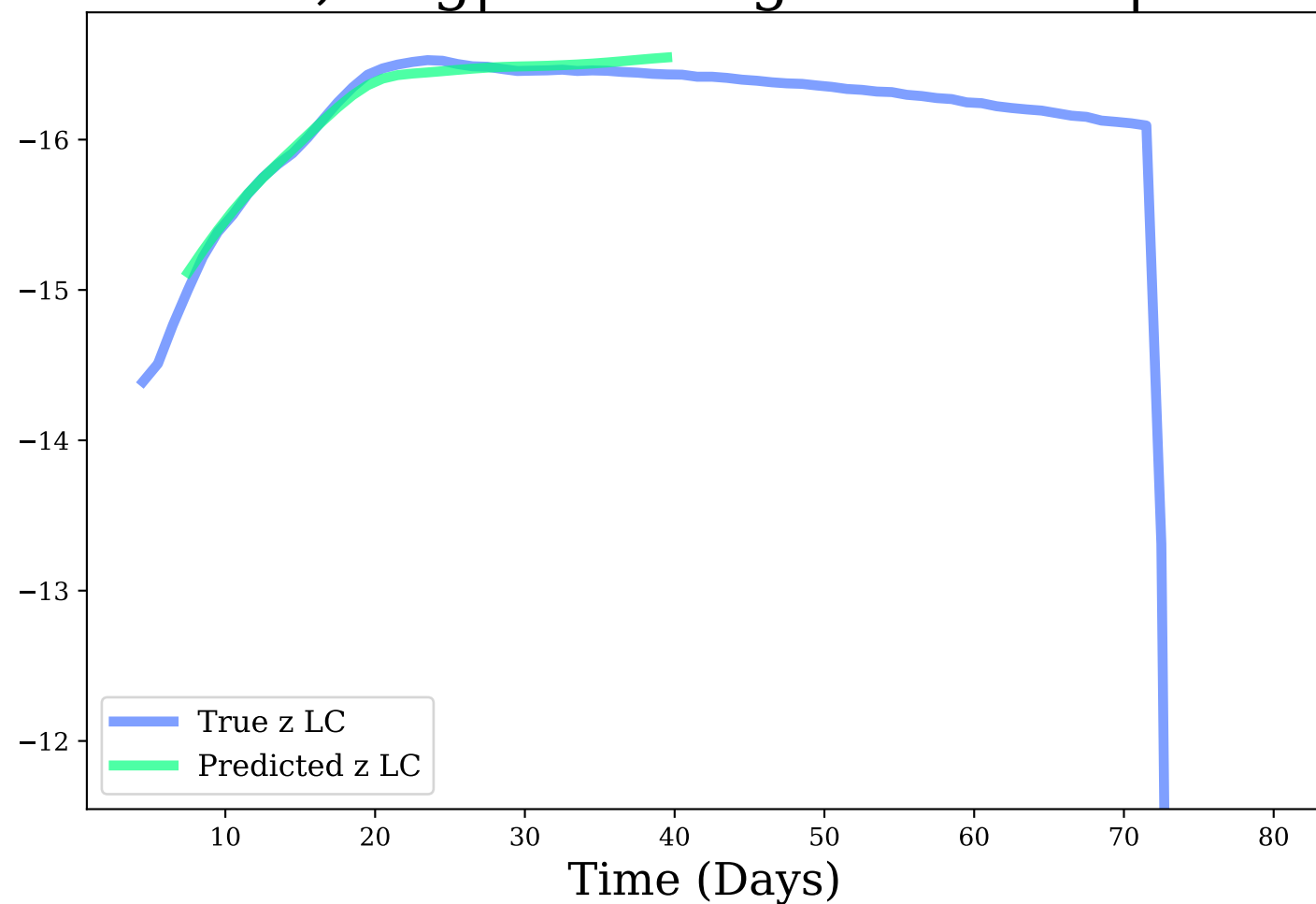
z-band, Avg|Max Mag Diff: 0.05 | 0.12
