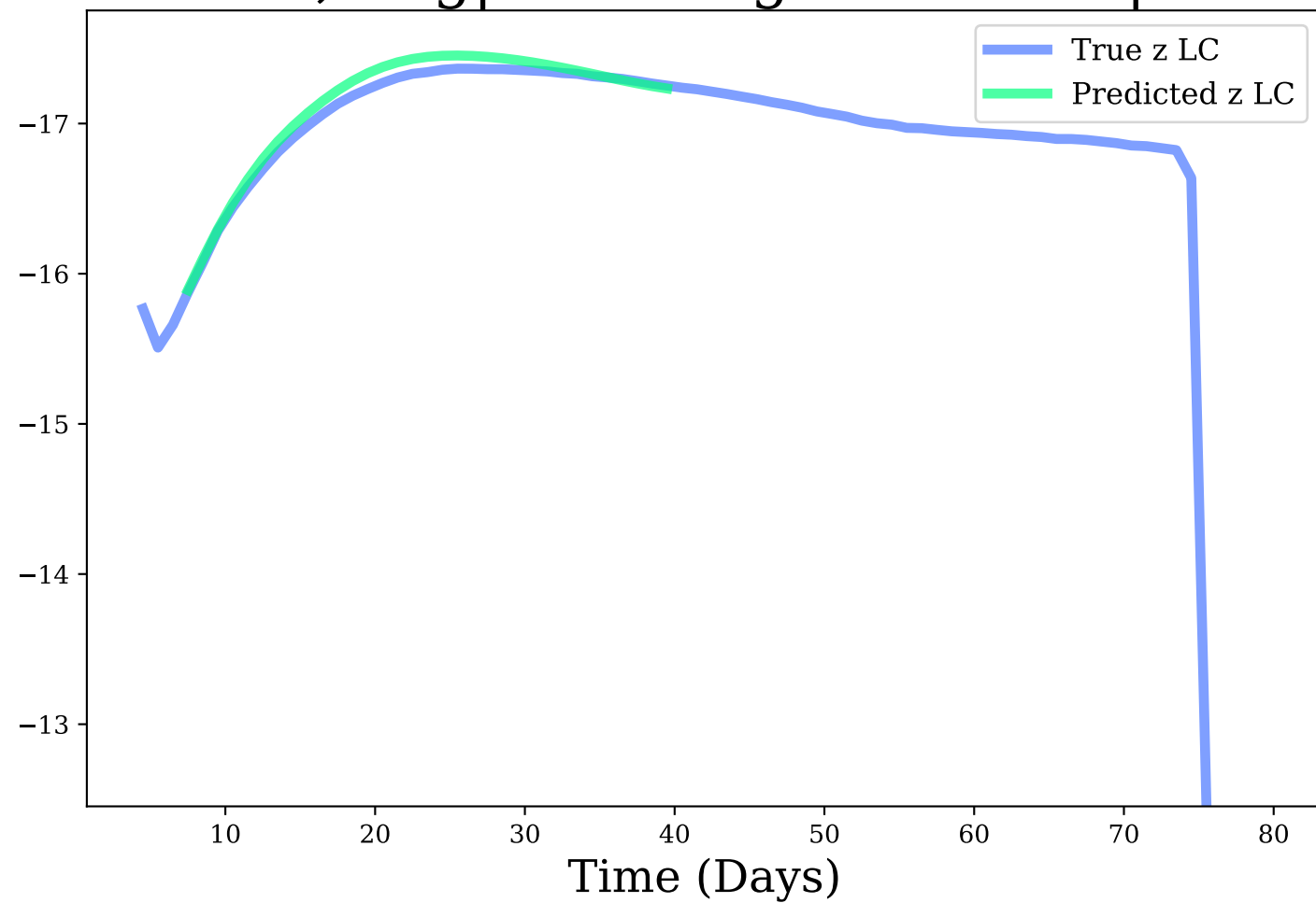
z-band, Avg|Max Mag Diff: 0.06 | 0.11
