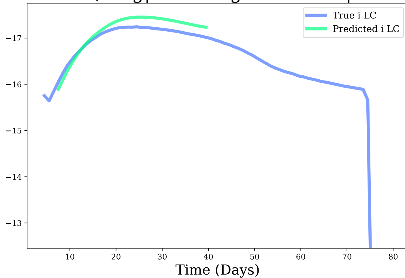
i-band, Avg|Max Mag Diff: 0.16 | 0.23
