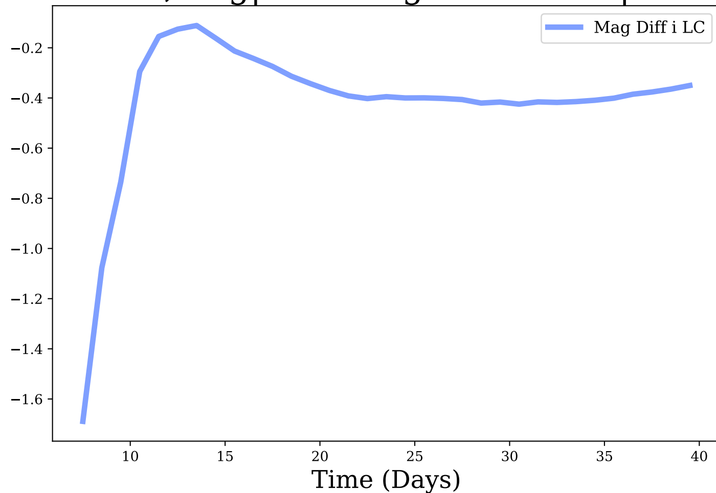
i-band, Avg|Max Mag Diff: -0.42 | 1.69
