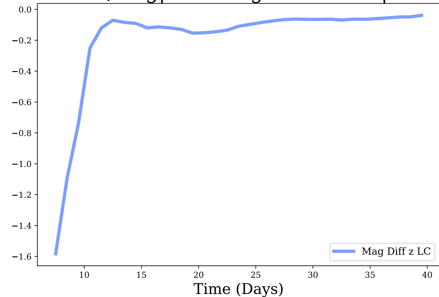
z-band, Avg|Max Mag Diff: -0.19 | 1.58
