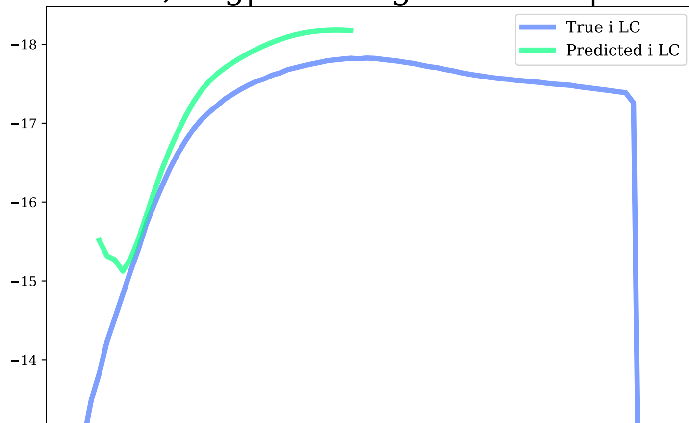
i-band, Avg|Max Mag Diff: 0.42 | 1.69
