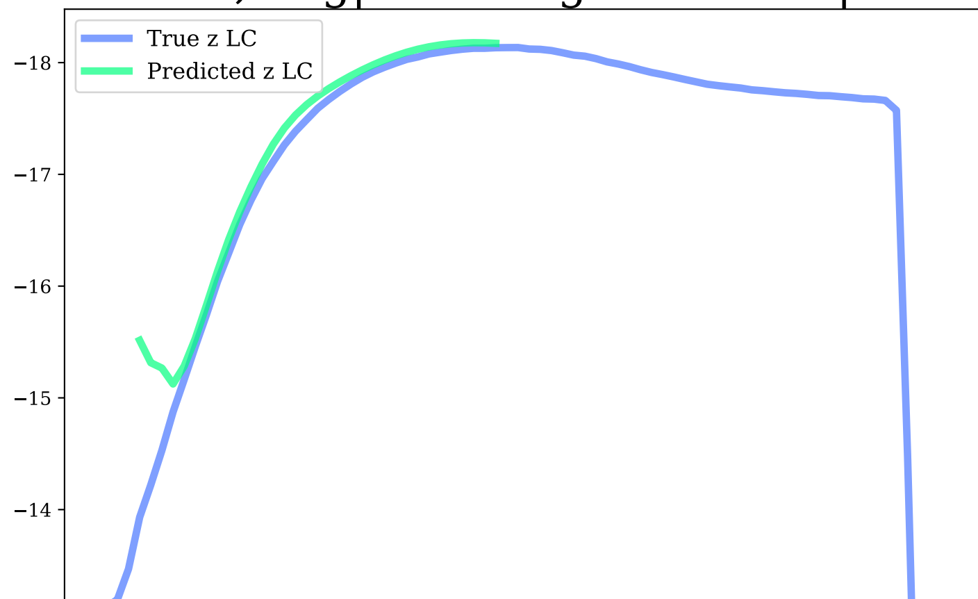
z-band, Avg|Max Mag Diff: 0.19 | 1.58
