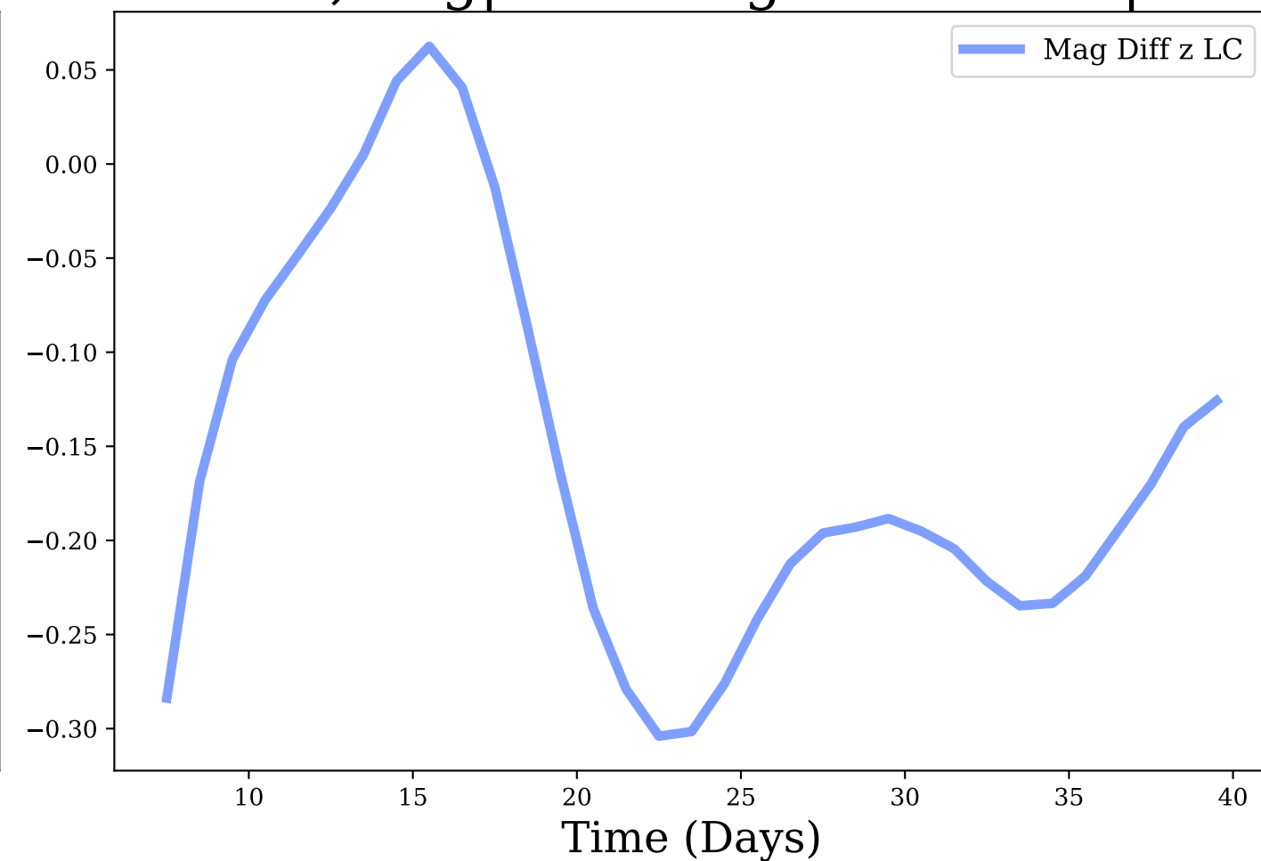
z-band, Avg|Max Mag Diff: -0.16 | 0.3
