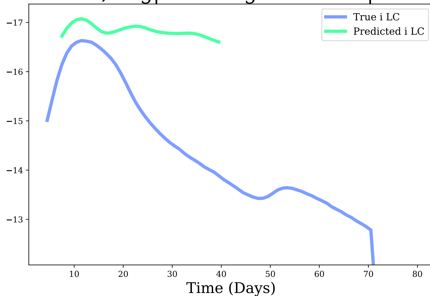
i-band, Avg|Max Mag Diff: 1.51 | 2.72
