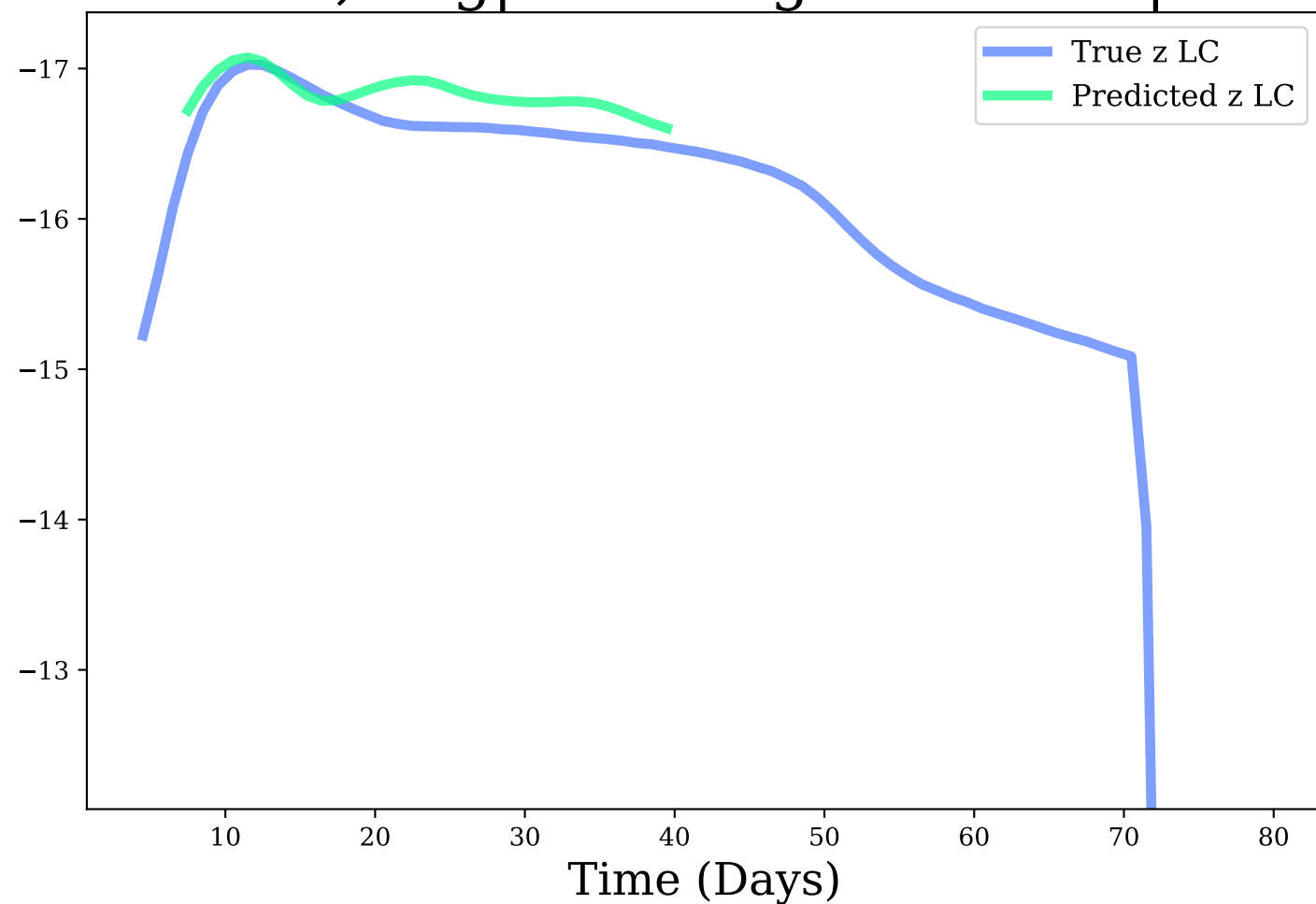
z-band, Avg|Max Mag Diff: 0.17 | 0.3
