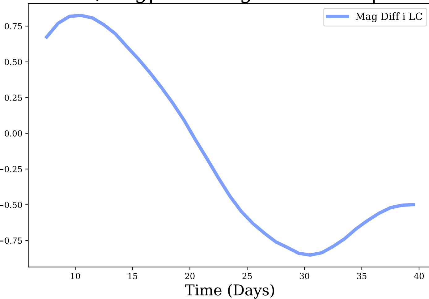
i-band, Avg|Max Mag Diff: -0.13 | 0.85
