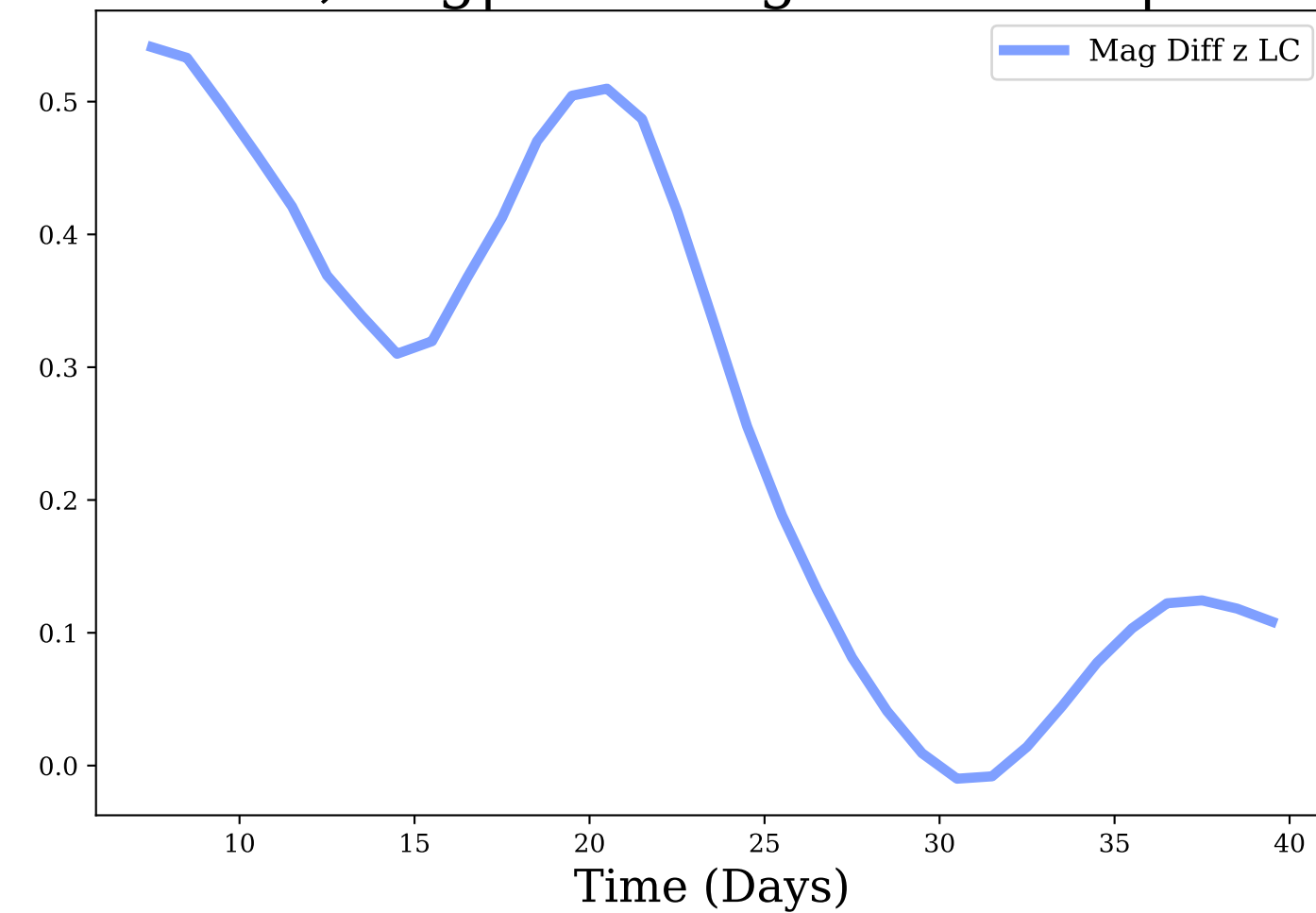
z-band, Avg|Max Mag Diff: 0.26 | 0.54
