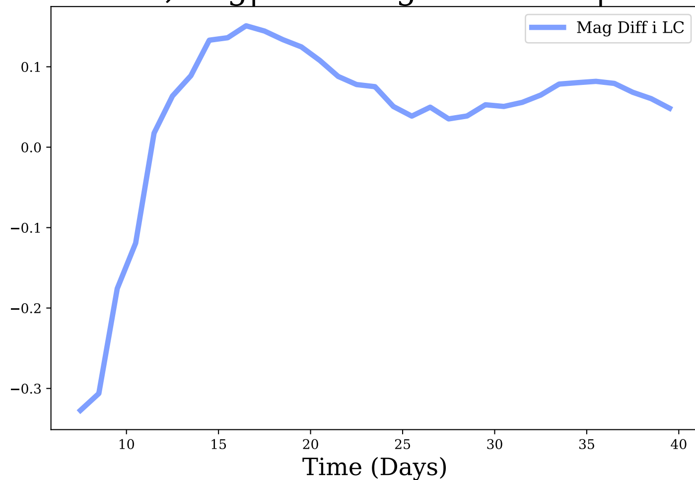
i-band, Avg|Max Mag Diff: 0.04 | 0.33
