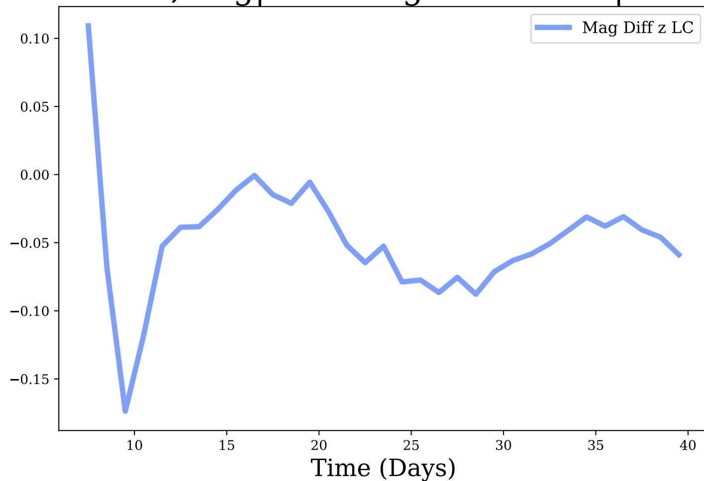
z-band, Avg|Max Mag Diff: -0.05 | 0.17
