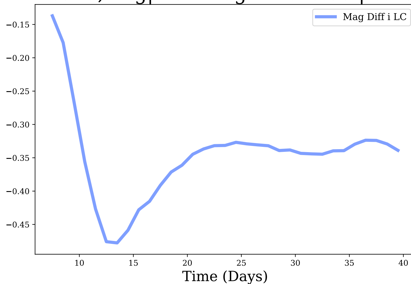
i-band, Avg|Max Mag Diff: -0.35 | 0.48
