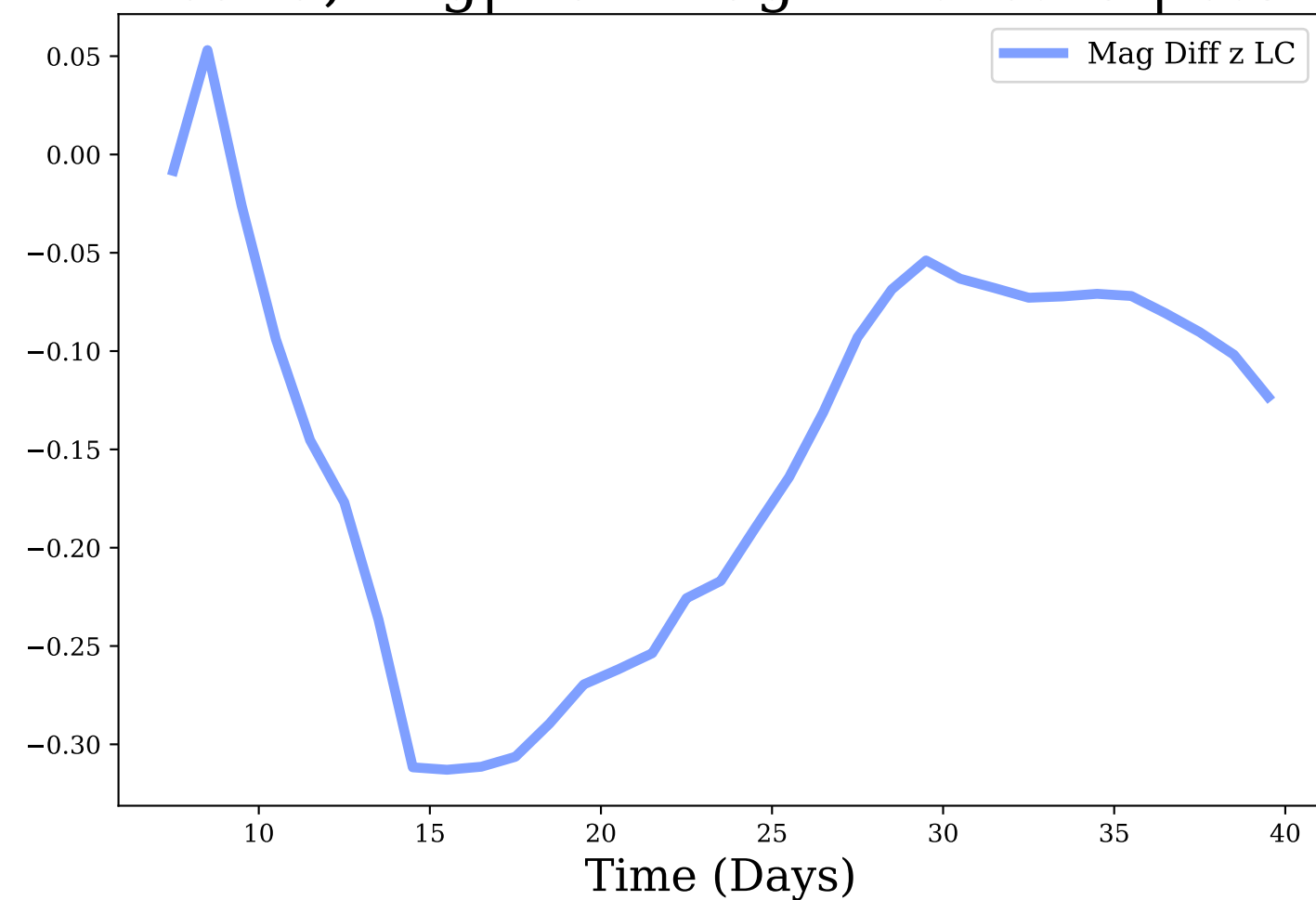
z-band, Avg|Max Mag Diff: -0.15 | 0.31
