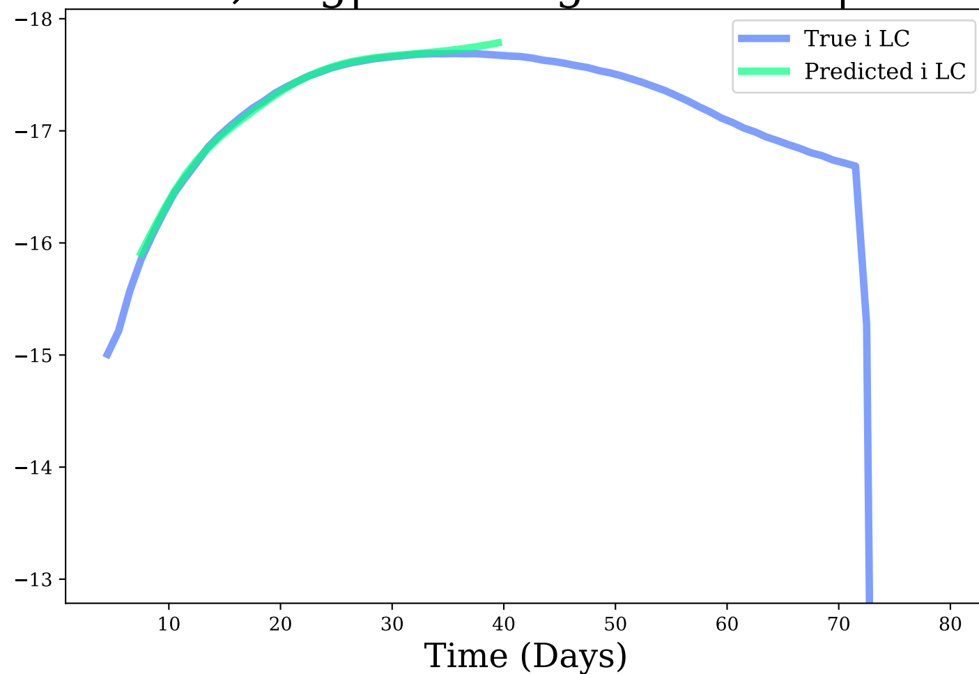
i-band, Avg|Max Mag Diff: 0.02 | 0.11
