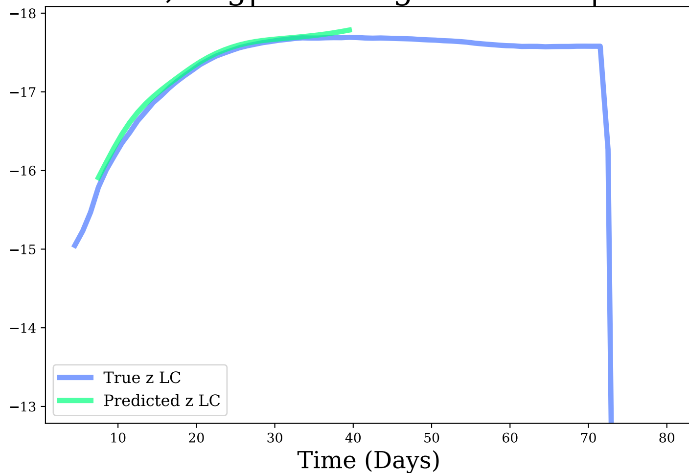
z-band, Avg|Max Mag Diff: 0.06 | 0.13
