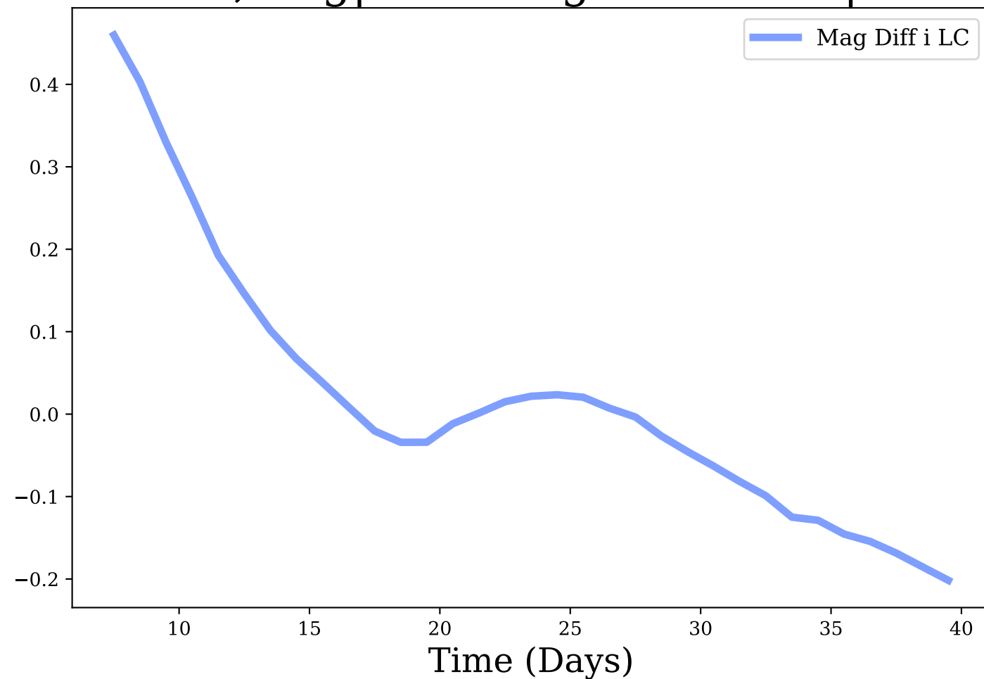
i-band, Avg|Max Mag Diff: 0.02 | 0.46
