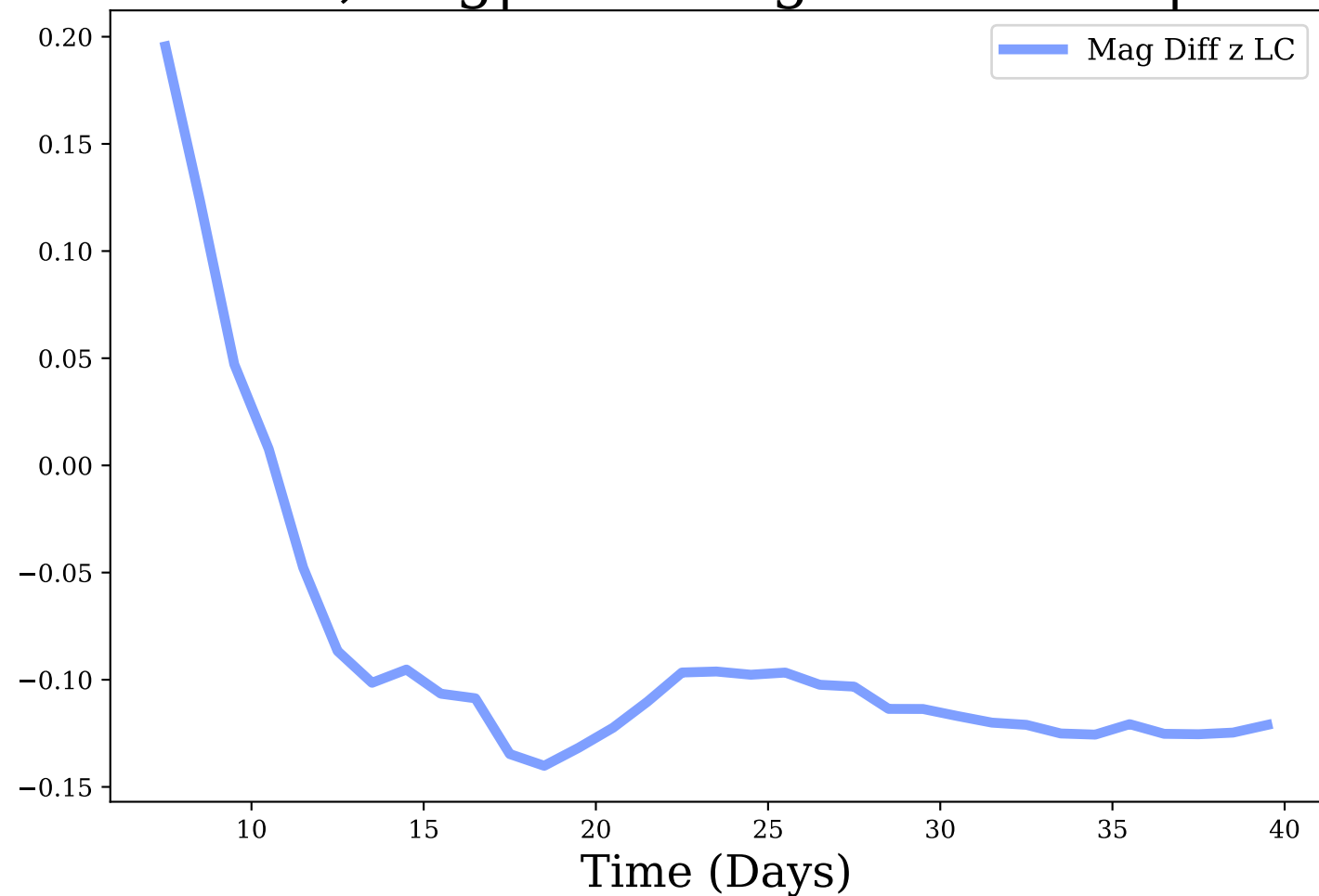
z-band, Avg|Max Mag Diff: -0.09 | 0.2
