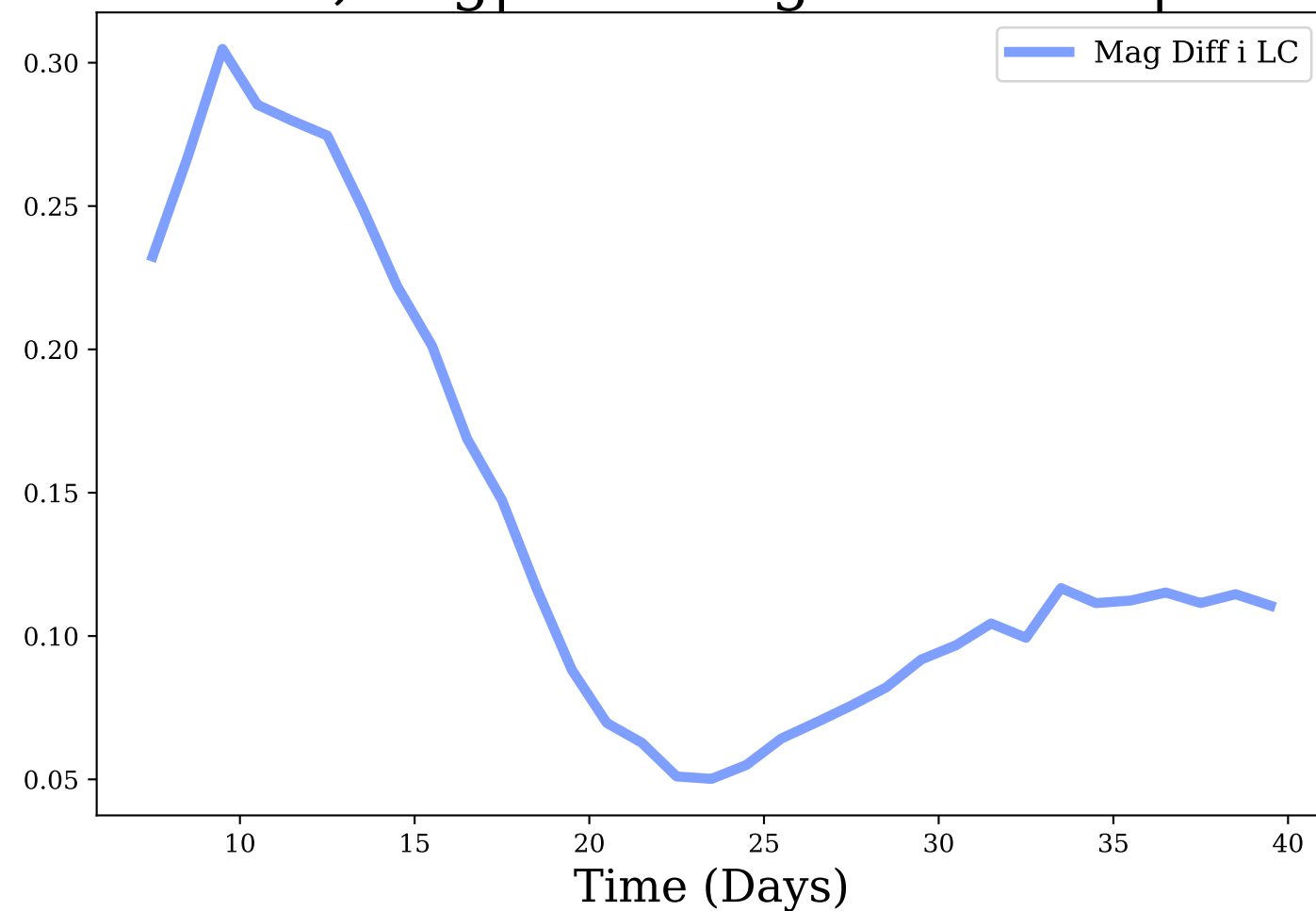
i-band, Avg|Max Mag Diff: 0.14 | 0.3
