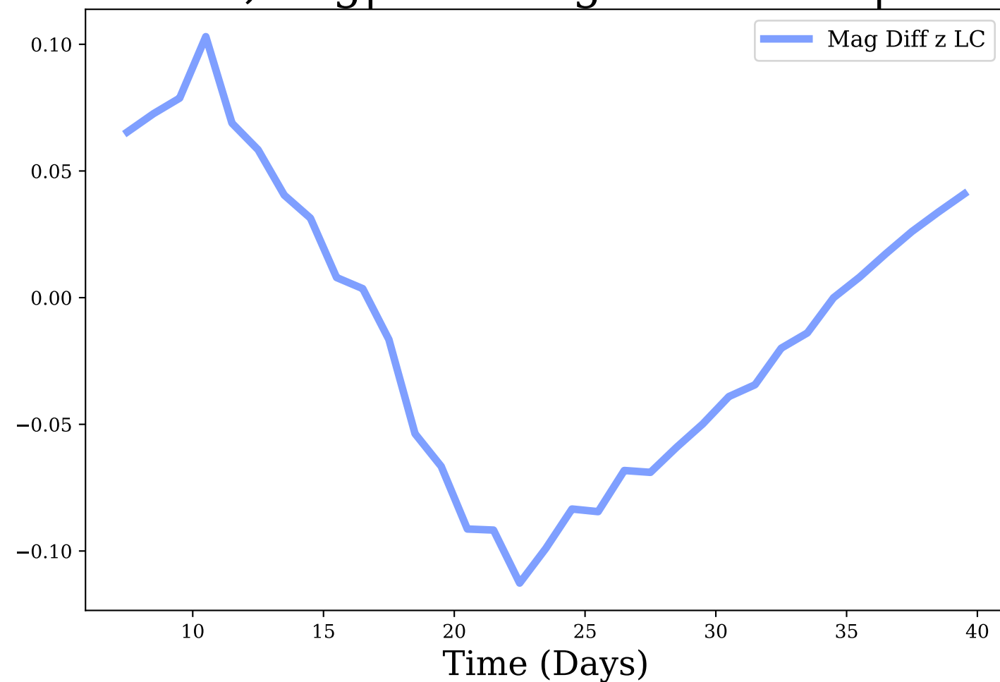
z-band, Avg|Max Mag Diff: -0.01 | 0.11
