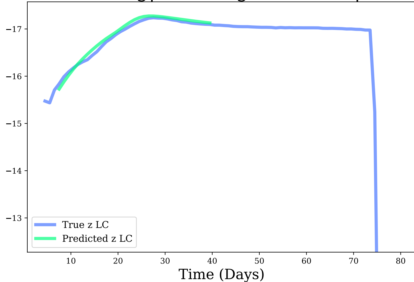
z-band, Avg|Max Mag Diff: 0.06 | 0.12
