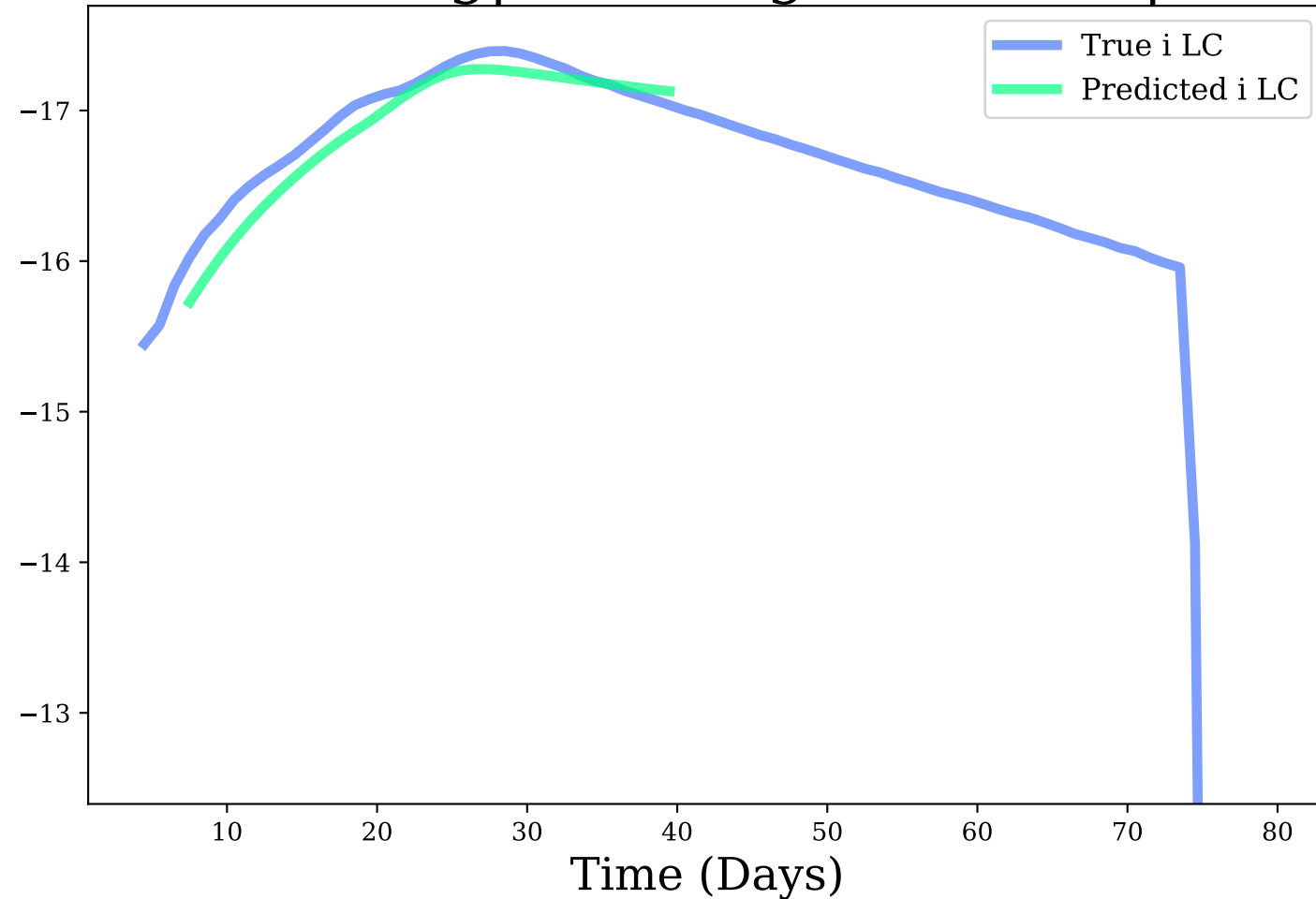
i-band, Avg|Max Mag Diff: 0.12 | 0.3
