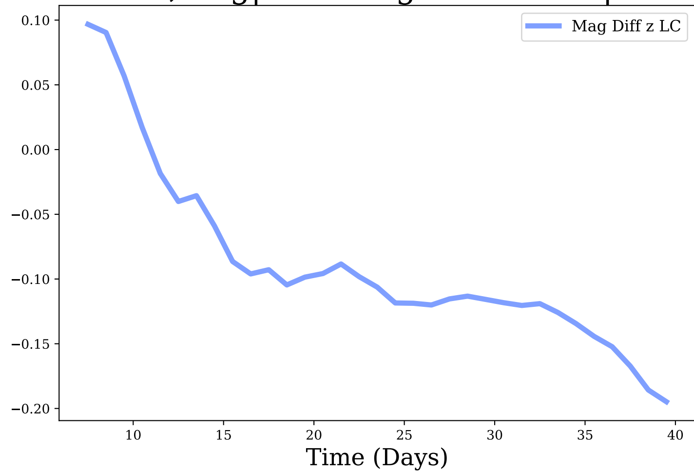
z-band, Avg|Max Mag Diff: -0.09 | 0.19
