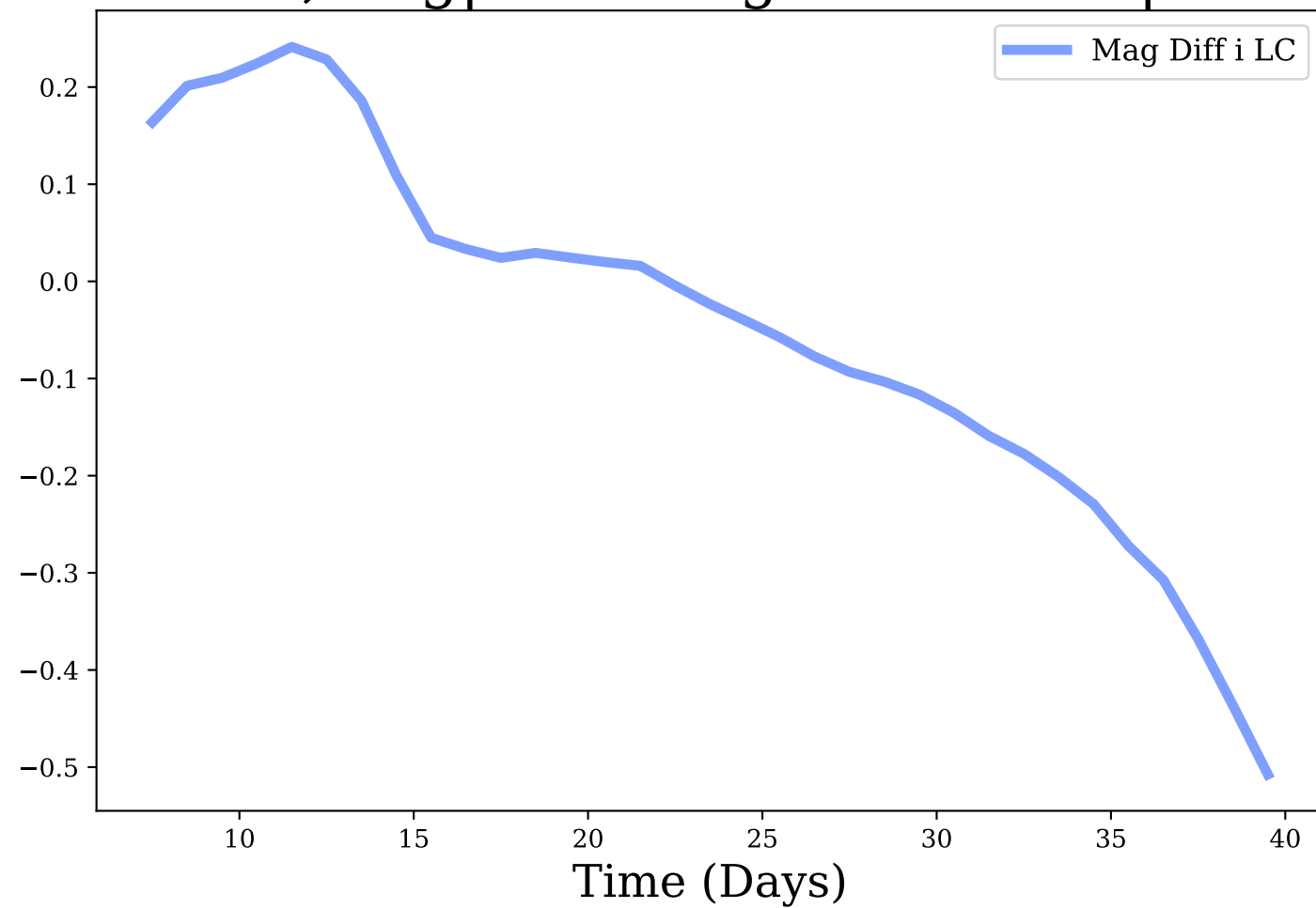
i-band, Avg|Max Mag Diff: -0.05 | 0.51
