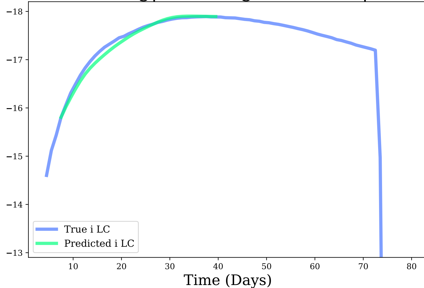
i-band, Avg|Max Mag Diff: 0.06 | 0.15
