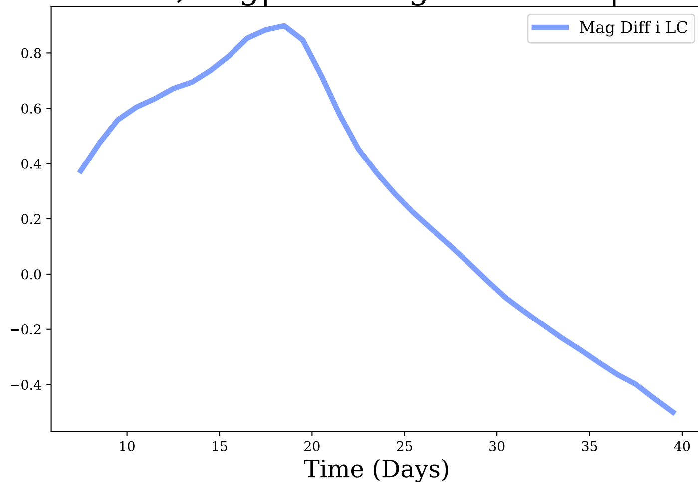
i-band, Avg|Max Mag Diff: 0.27 | 0.9
