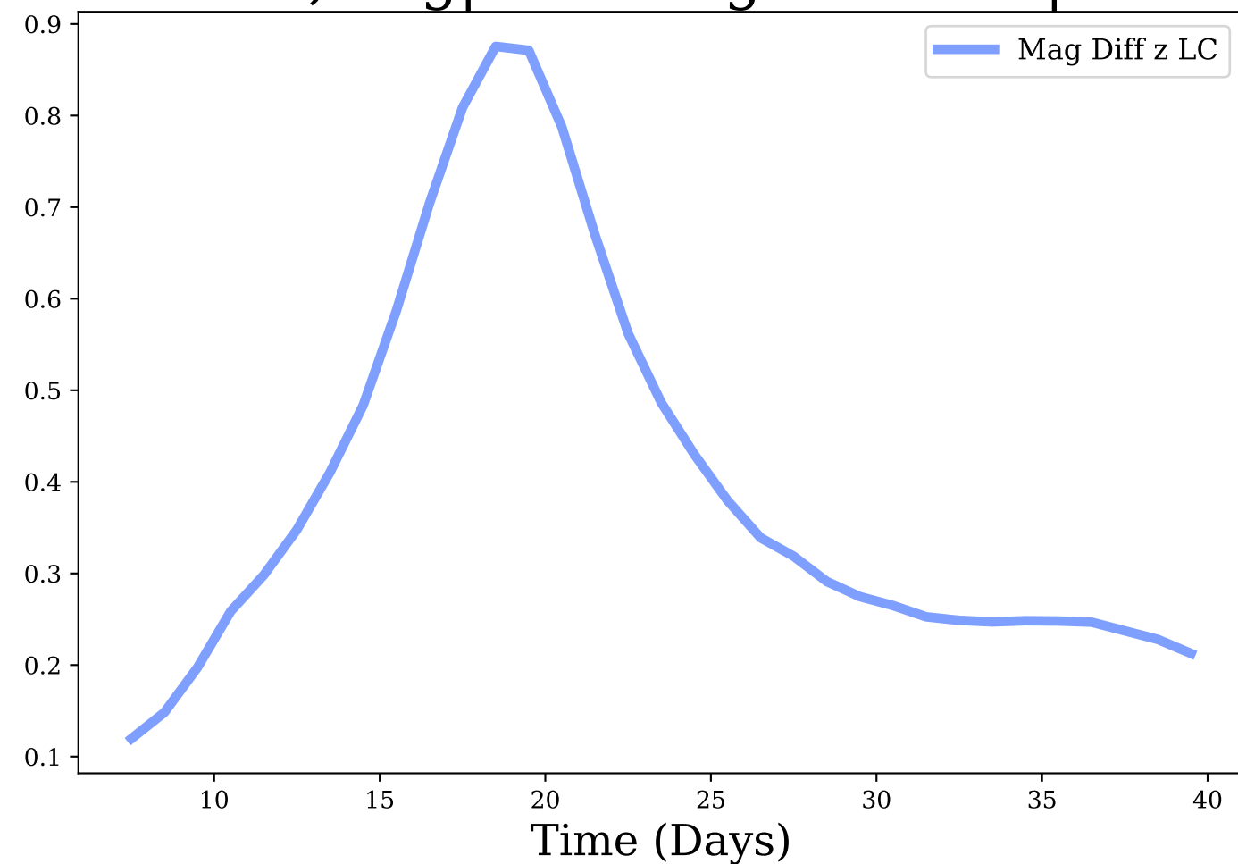
z-band, Avg|Max Mag Diff: 0.4 | 0.88
