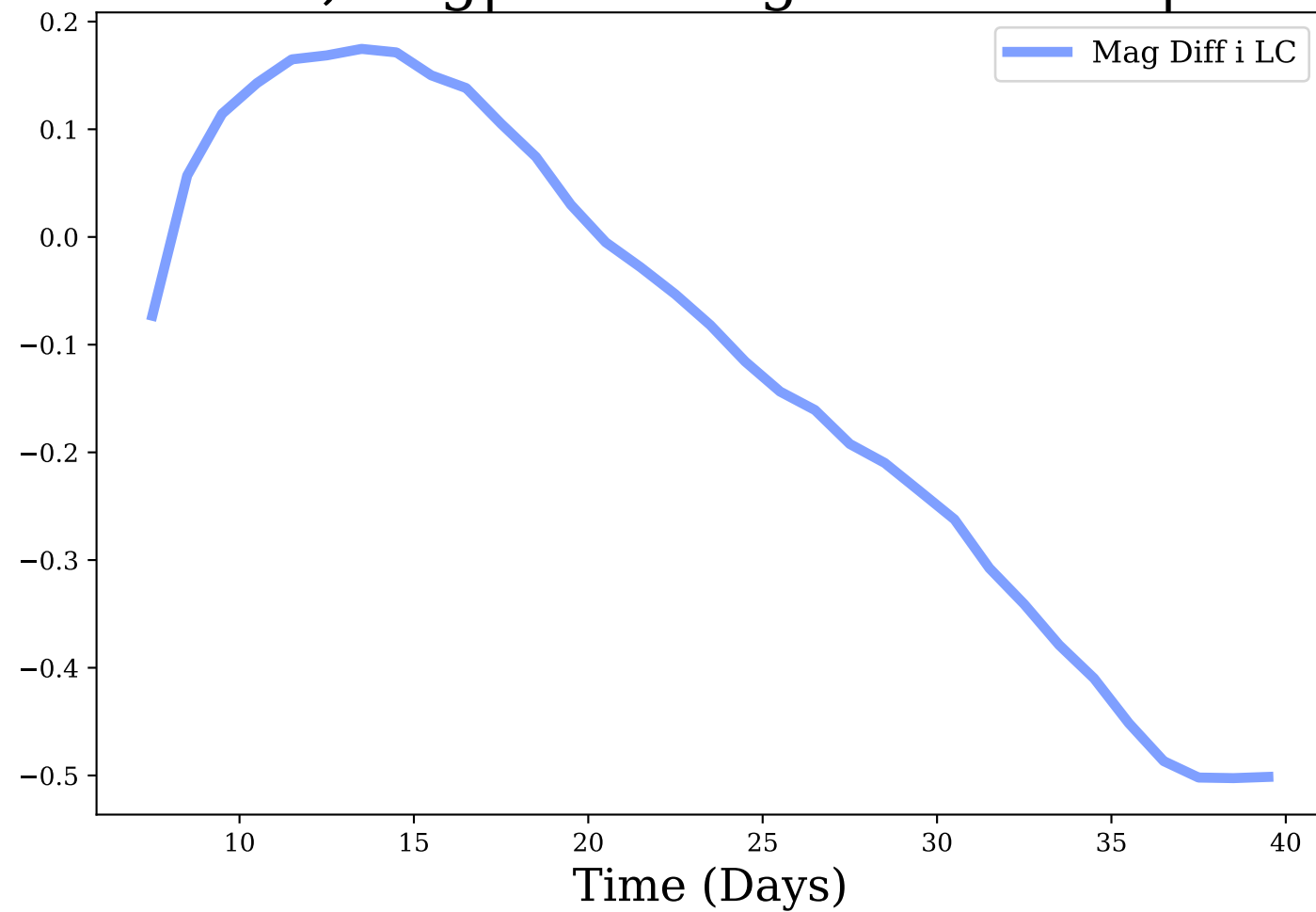
i-band, Avg|Max Mag Diff: -0.12 | 0.5
