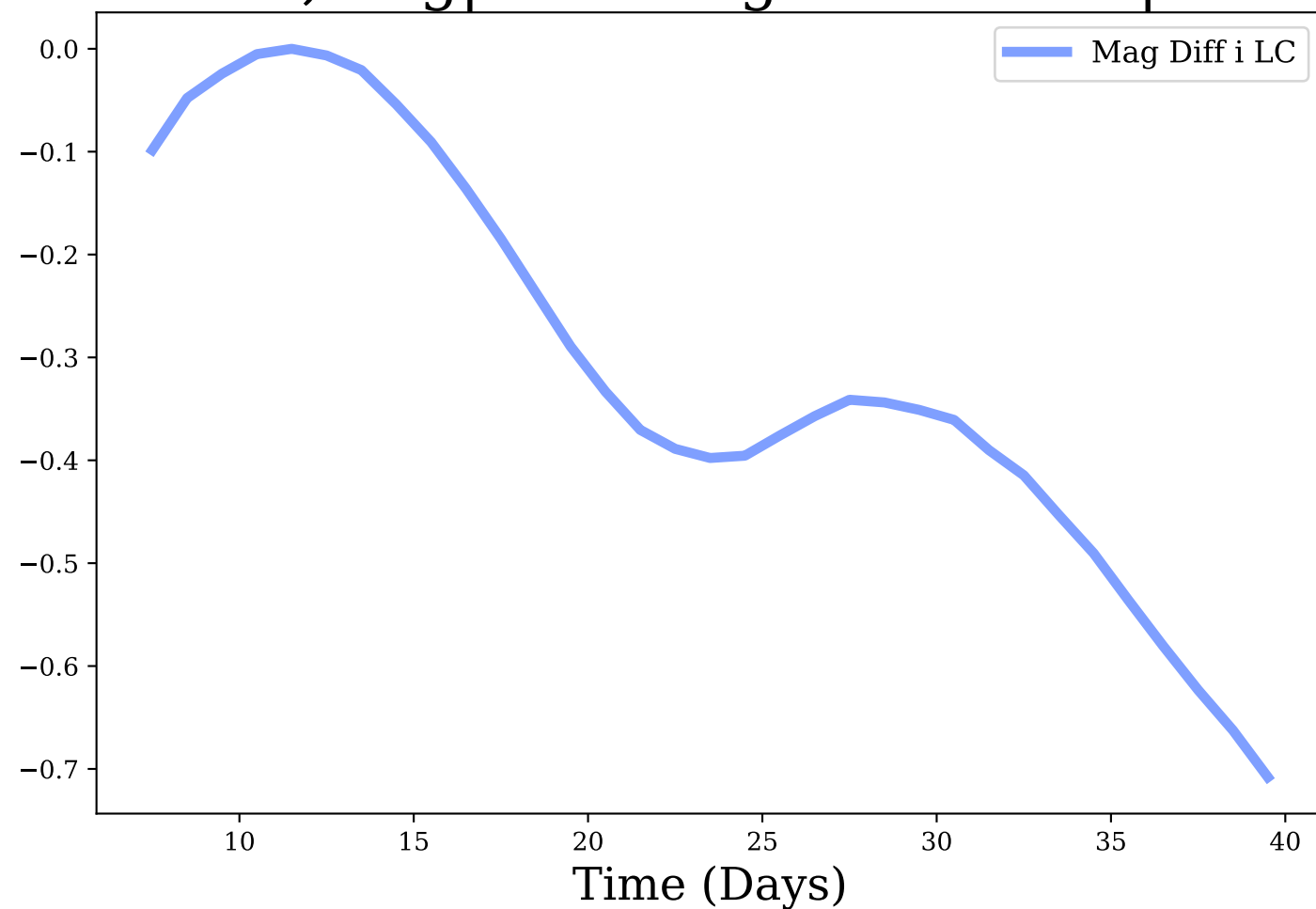
i-band, Avg|Max Mag Diff: -0.31 | 0.71
