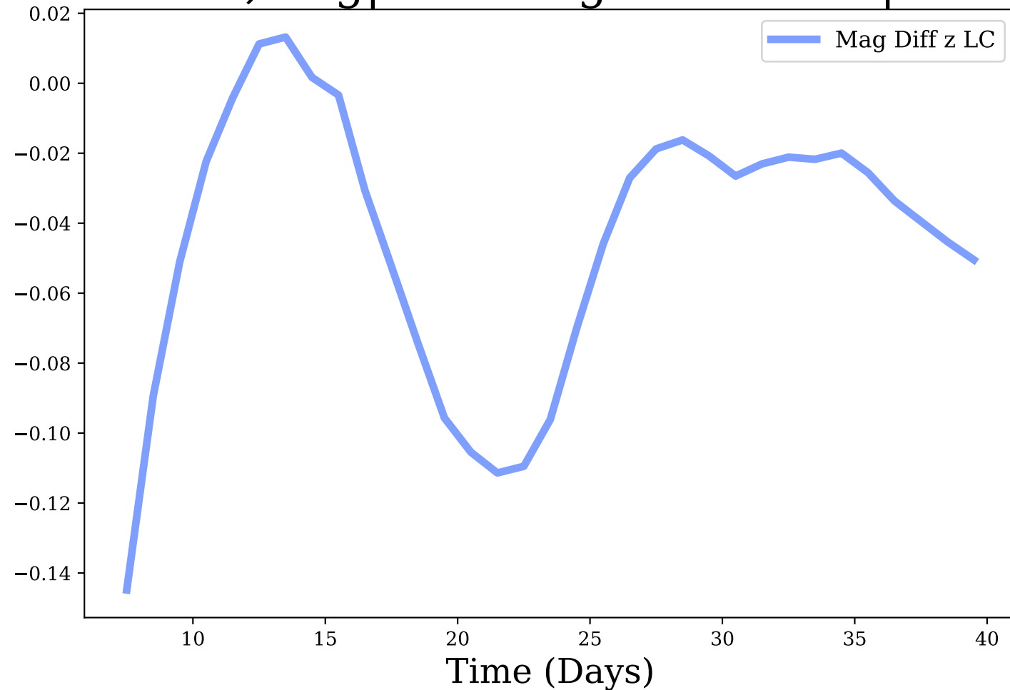
z-band, Avg|Max Mag Diff: -0.04 | 0.14
