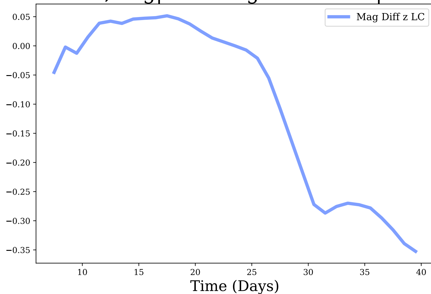
z-band, Avg|Max Mag Diff: -0.09 | 0.35
