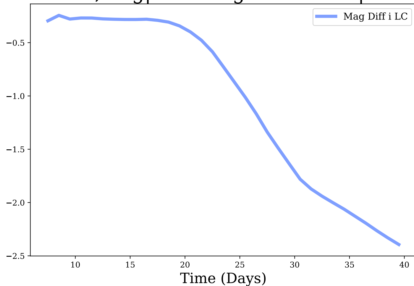
i-band, Avg|Max Mag Diff: -1.04 | 2.39
