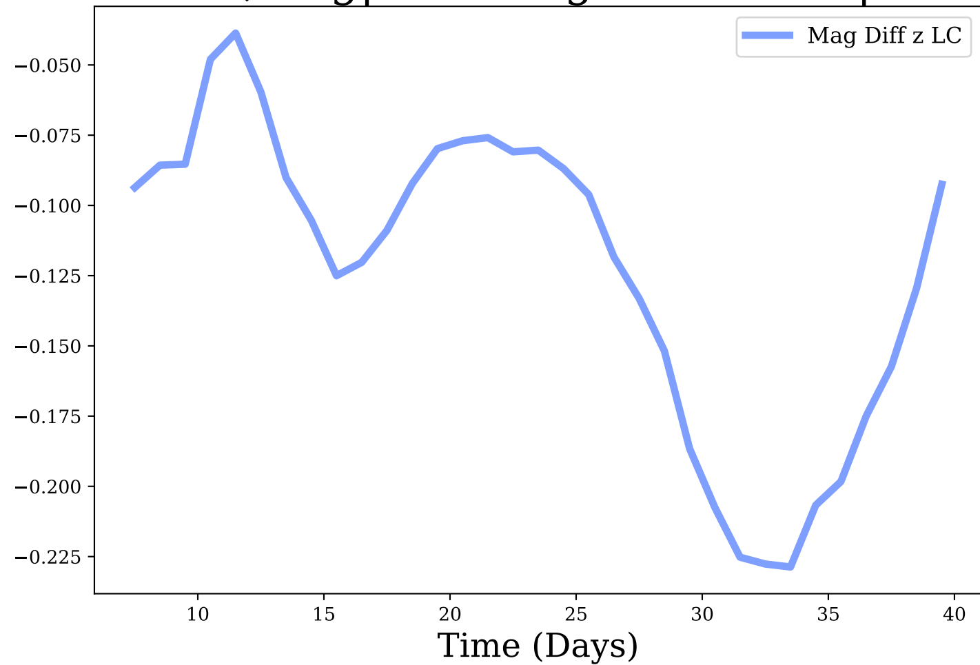
z-band, Avg|Max Mag Diff: -0.12 | 0.23
