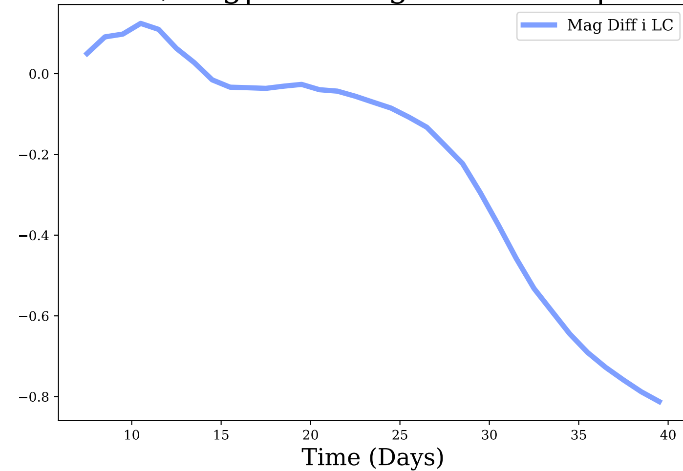
i-band, Avg|Max Mag Diff: -0.22 | 0.81
