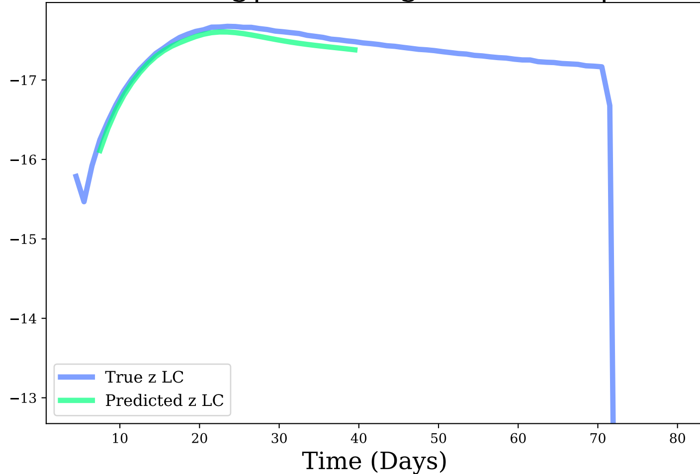
z-band, Avg|Max Mag Diff: 0.08 | 0.14
