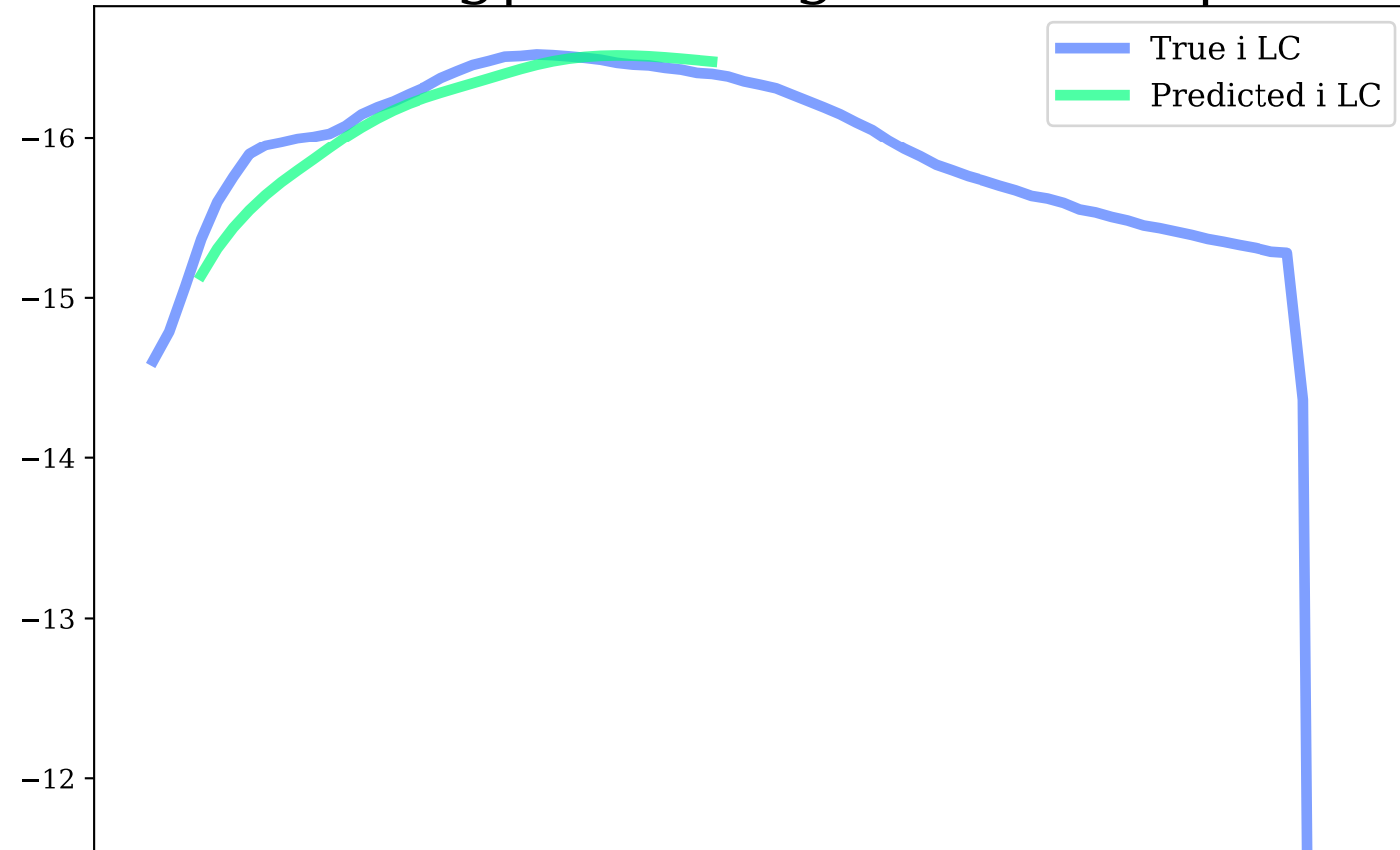
i-band, Avg|Max Mag Diff: 0.11 | 0.35
