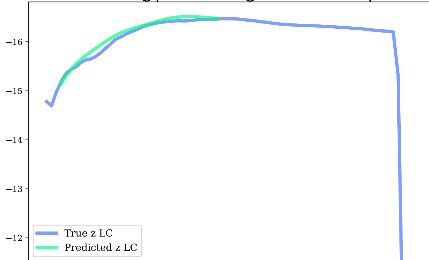
z-band, Avg|Max Mag Diff: 0.07 | 0.17
