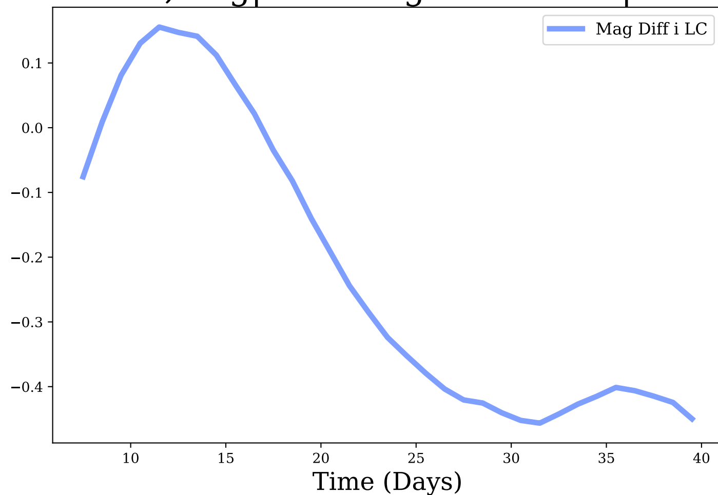
i-band, Avg|Max Mag Diff: -0.22 | 0.46
