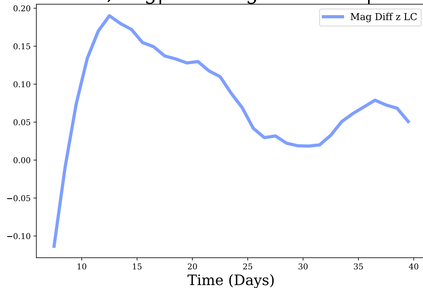
z-band, Avg|Max Mag Diff: 0.08 | 0.19
