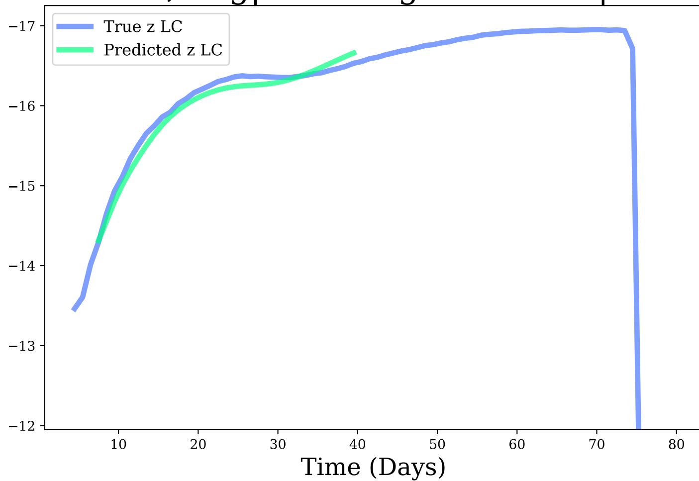
z-band, Avg|Max Mag Diff: 0.09 | 0.15
