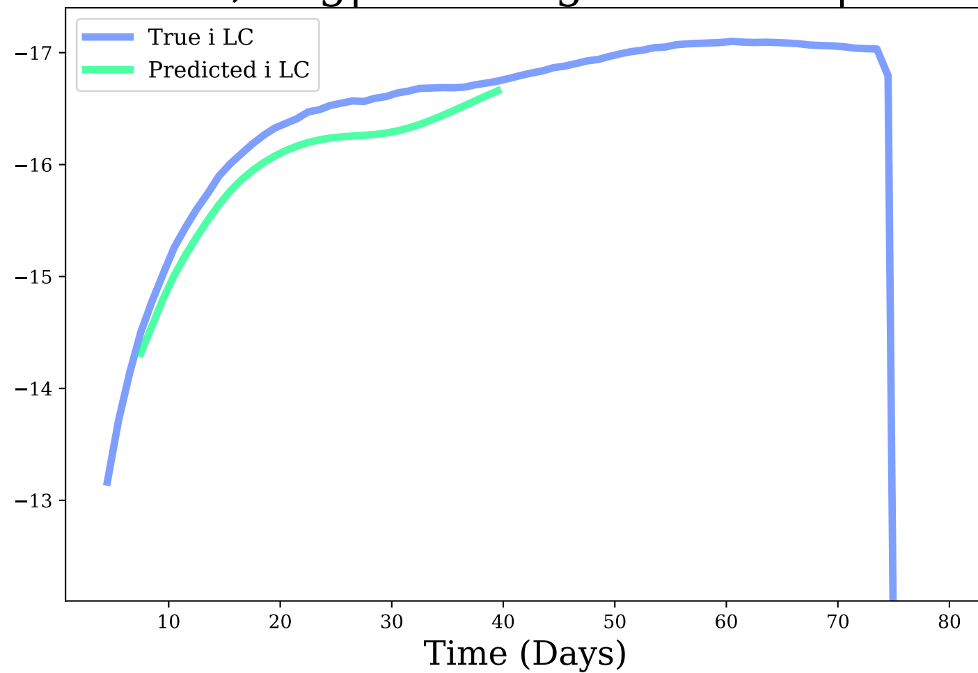
i-band, Avg|Max Mag Diff: 0.25 | 0.34
