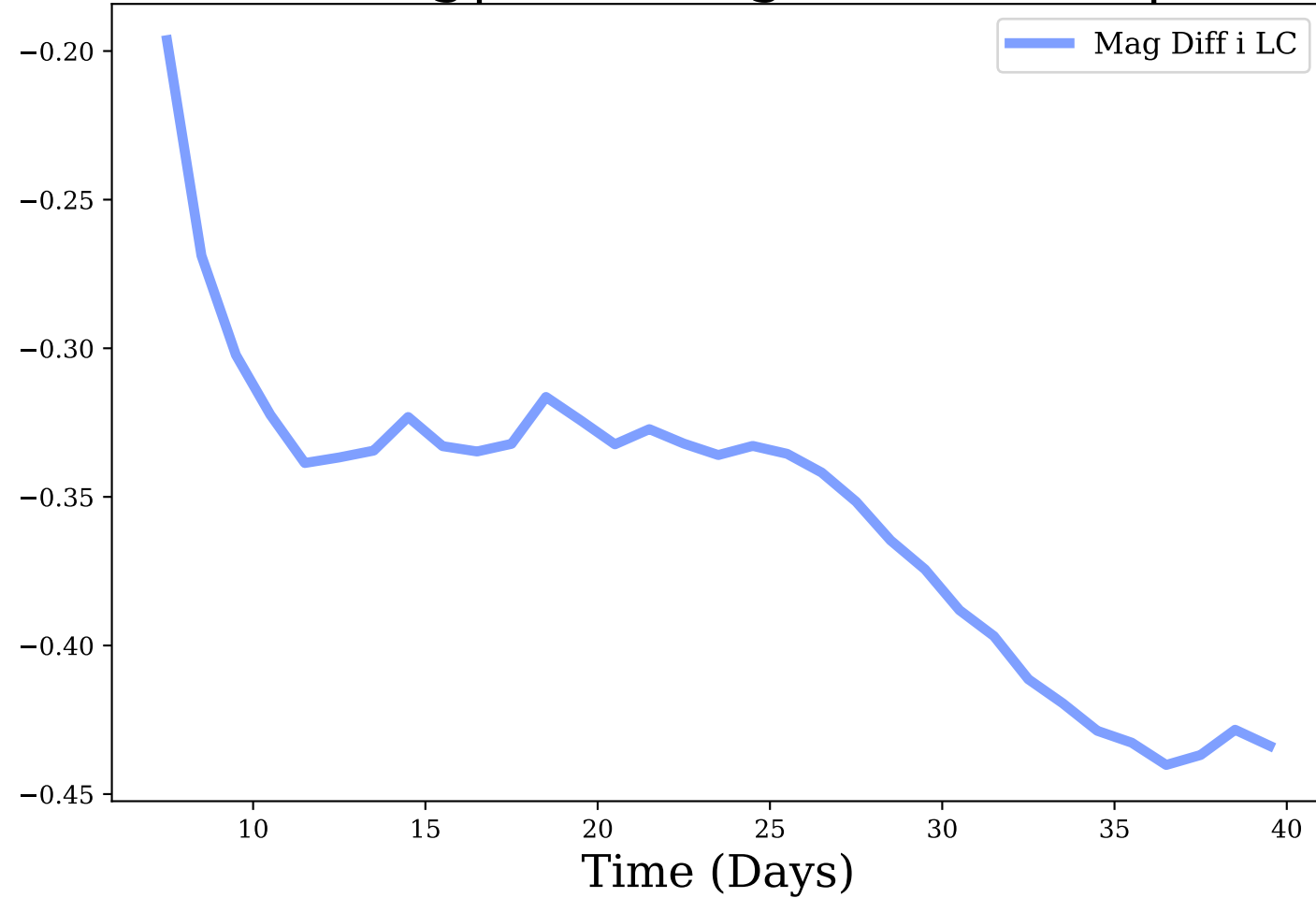
i-band, Avg|Max Mag Diff: -0.35 | 0.44
