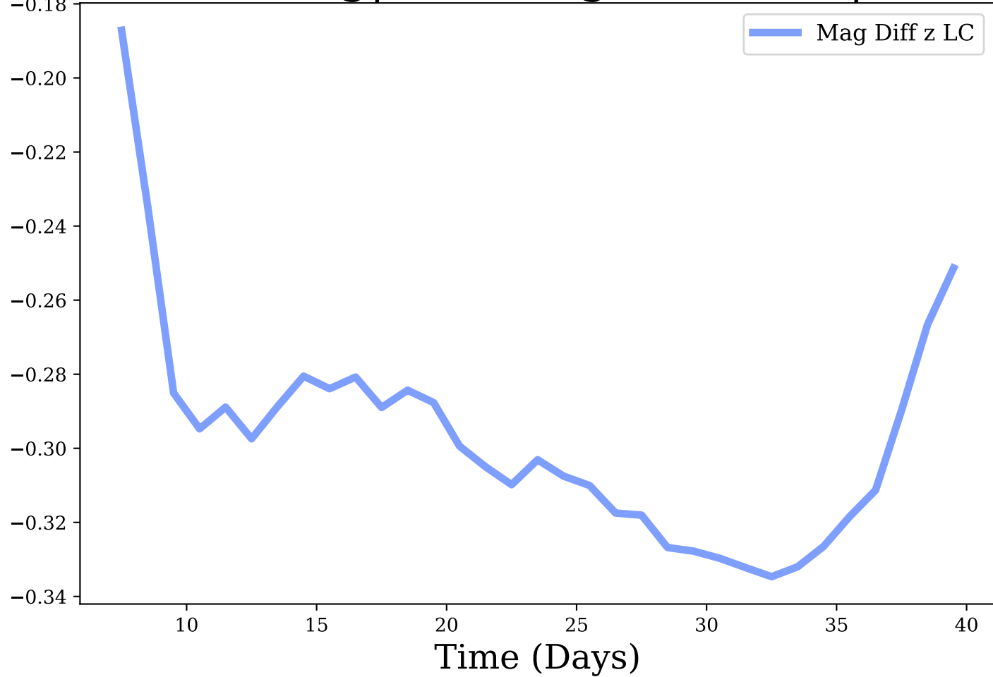
z-band, Avg|Max Mag Diff: -0.3 | 0.33
