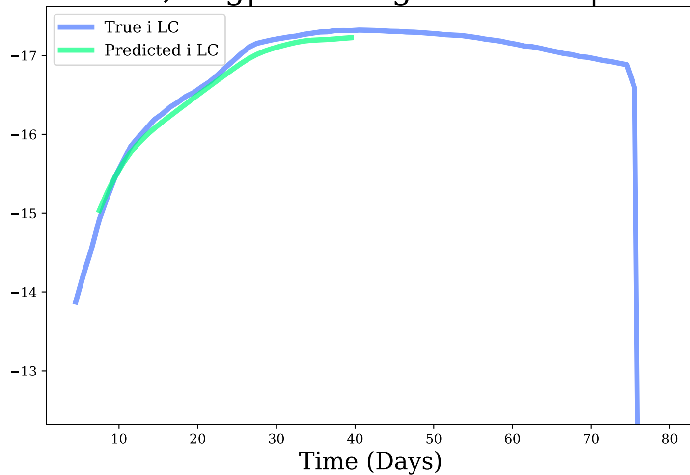
i-band, Avg|Max Mag Diff: 0.09 | 0.14
