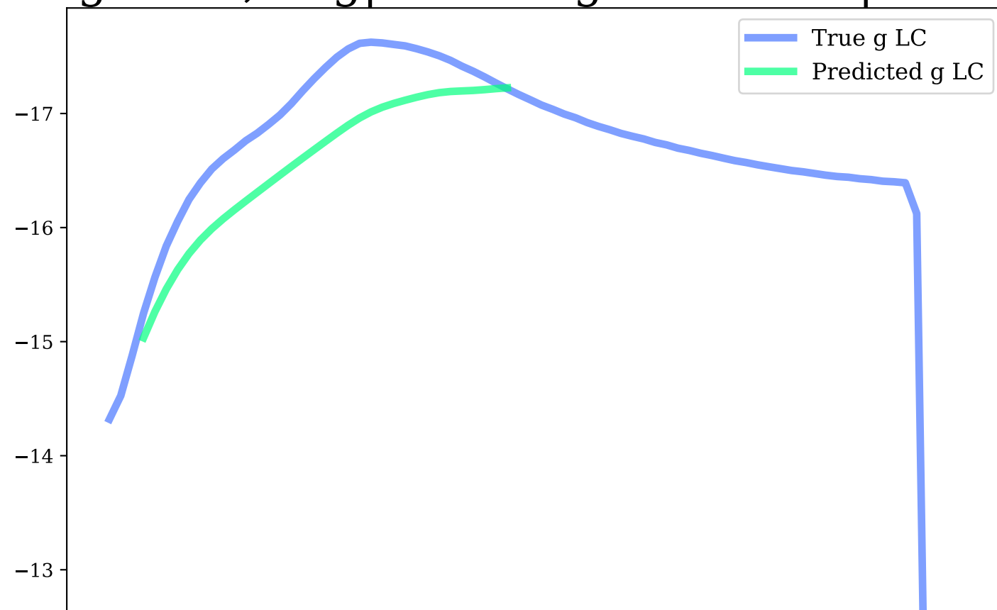
i-band, Avg|Max Mag Diff: 0.09 | 0.14
