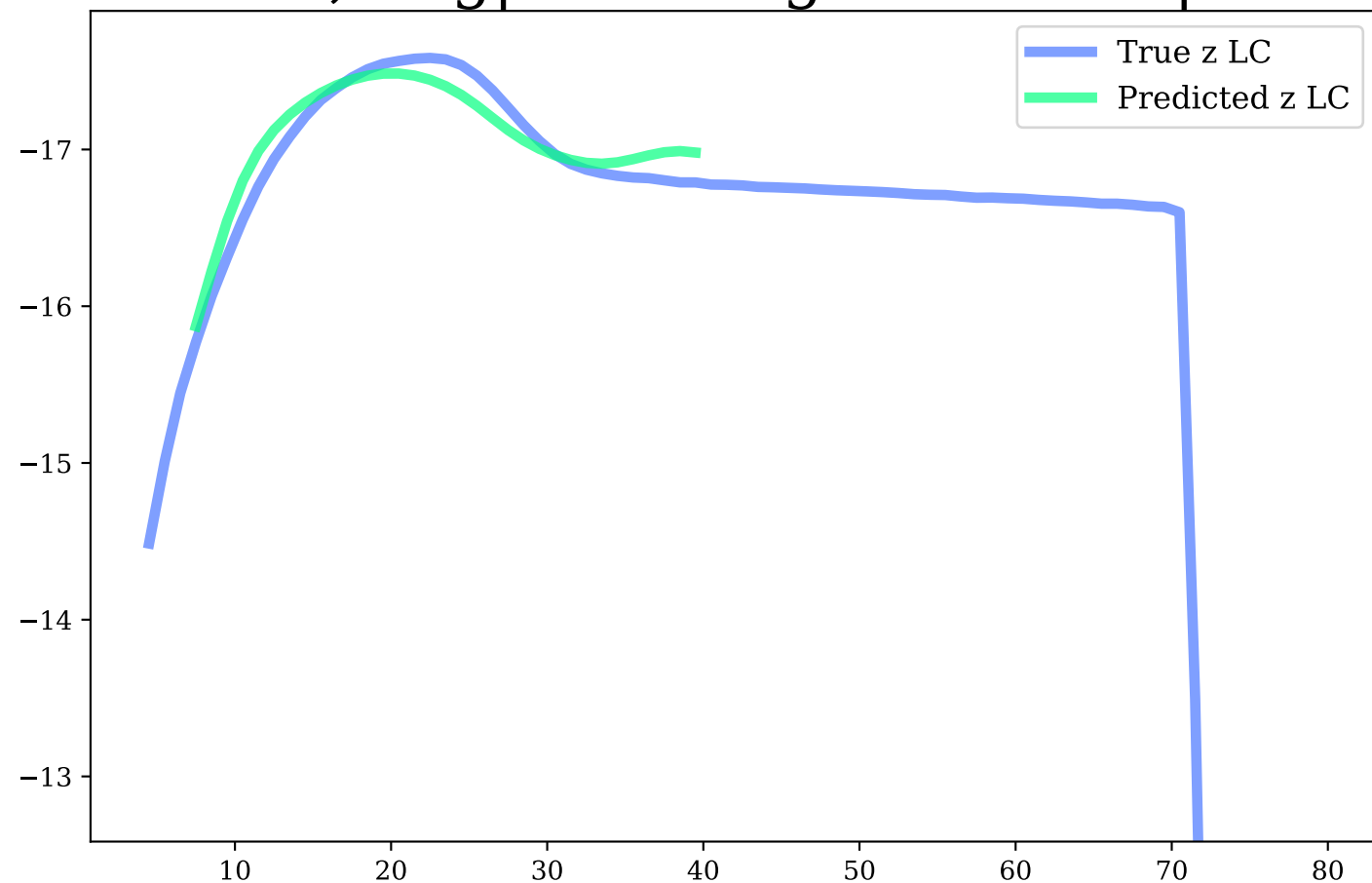
z-band, Avg|Max Mag Diff: 0.12 | 0.25
