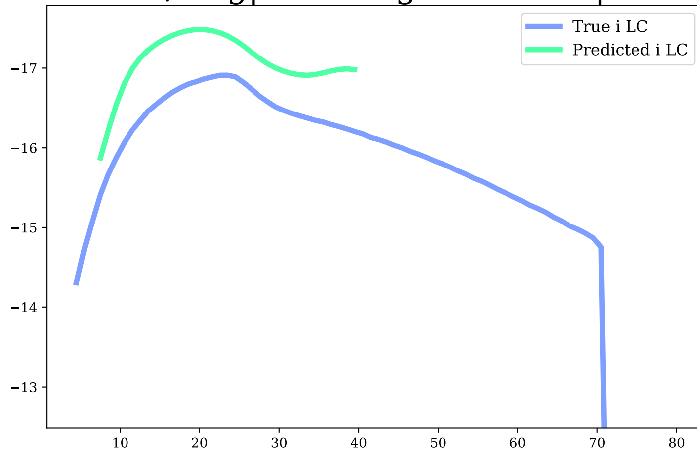
i-band, Avg|Max Mag Diff: 0.61 | 0.78
