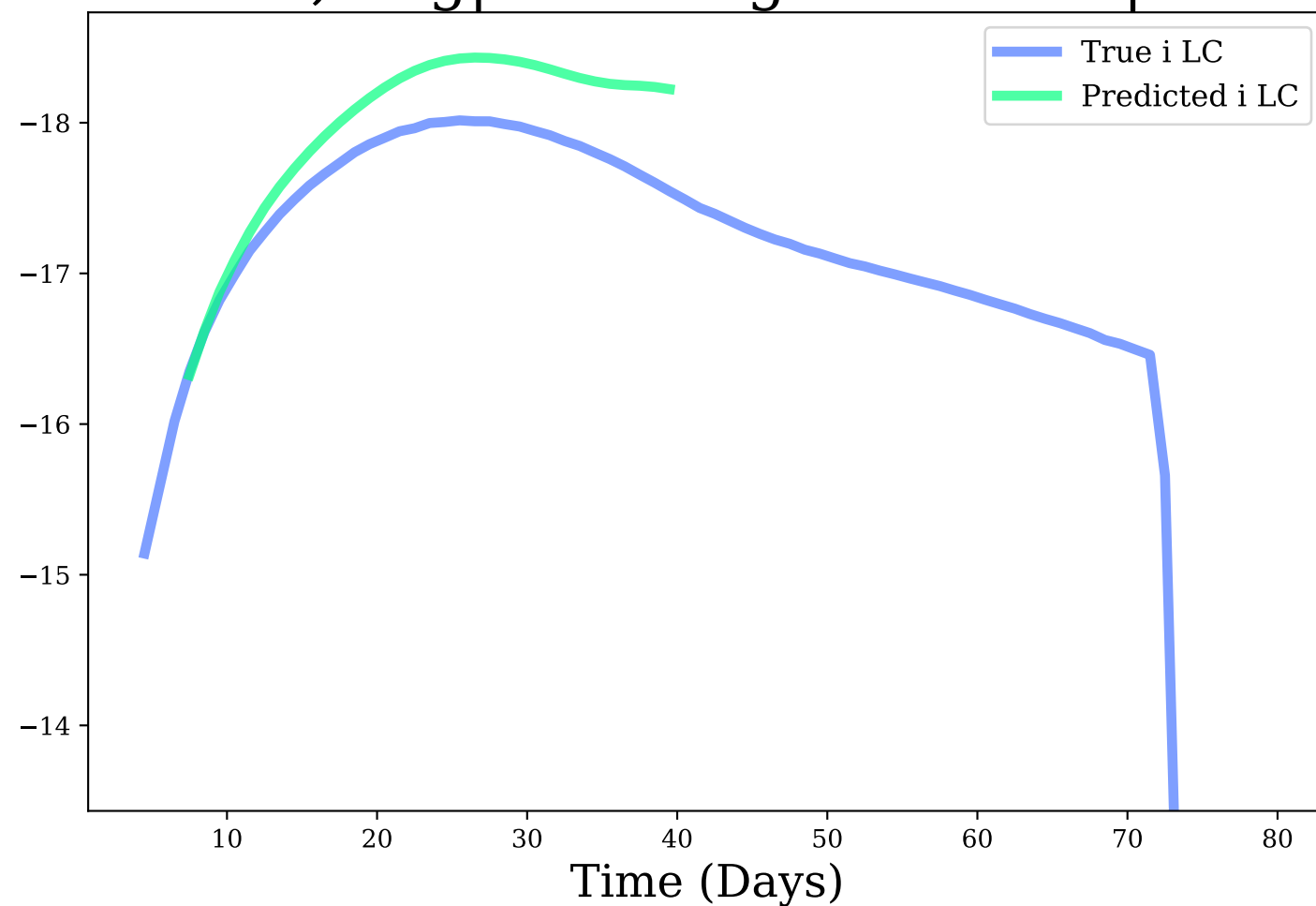
i-band, Avg|Max Mag Diff: 0.34 | 0.68
