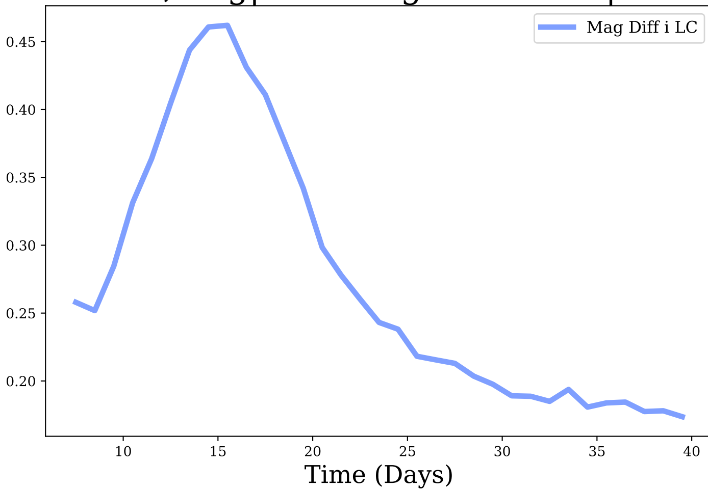
i-band, Avg|Max Mag Diff: 0.27 | 0.46
