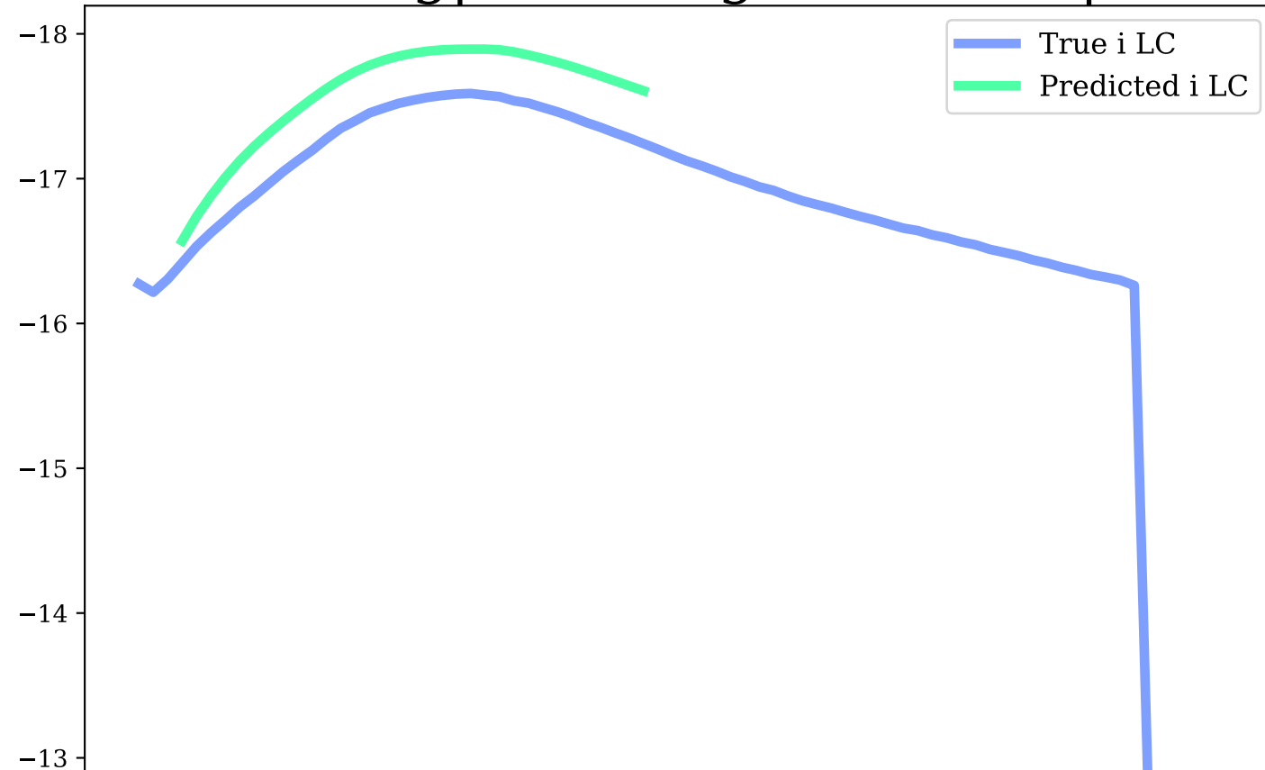
i-band, Avg|Max Mag Diff: 0.32 | 0.37
