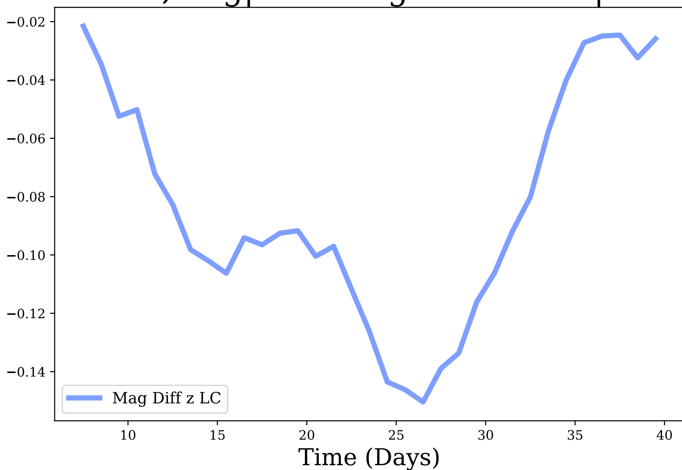
z-band, Avg|Max Mag Diff: -0.08 | 0.15
