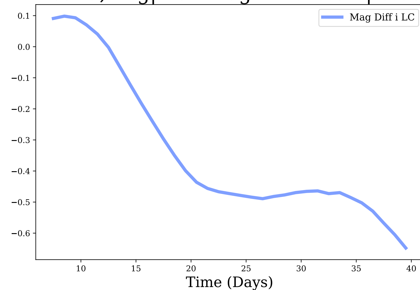
i-band, Avg|Max Mag Diff: -0.34 | 0.65
