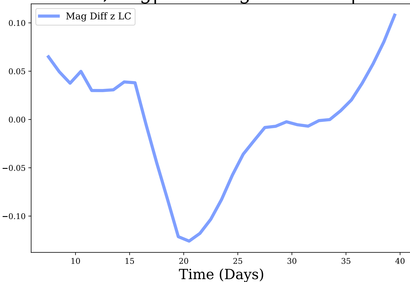
z-band, Avg|Max Mag Diff: -0.0 | 0.13
