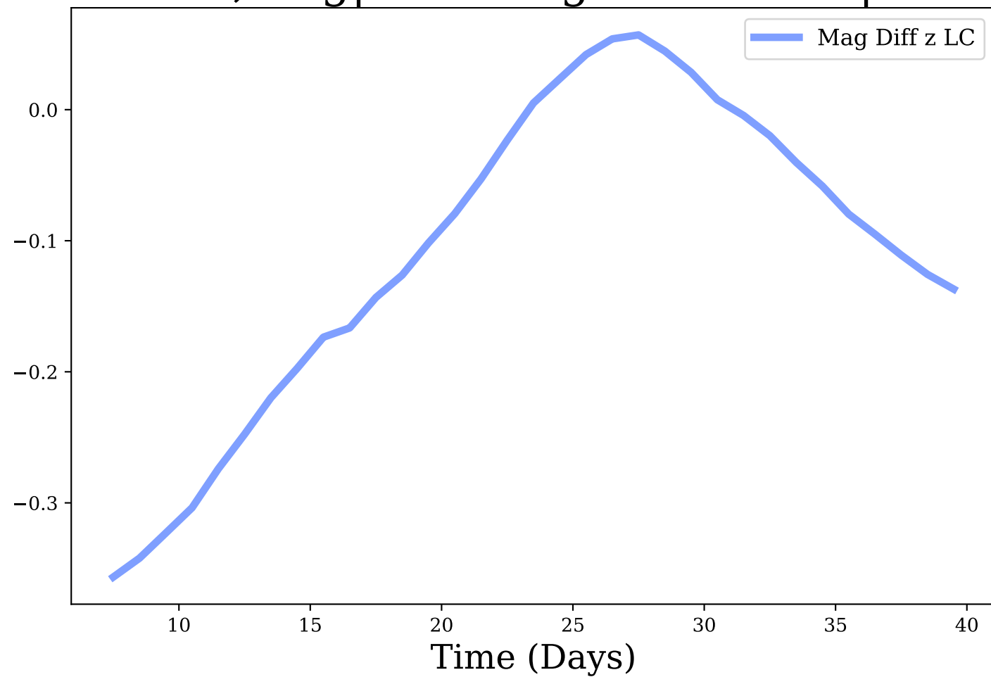
z-band, Avg|Max Mag Diff: -0.11 | 0.36
