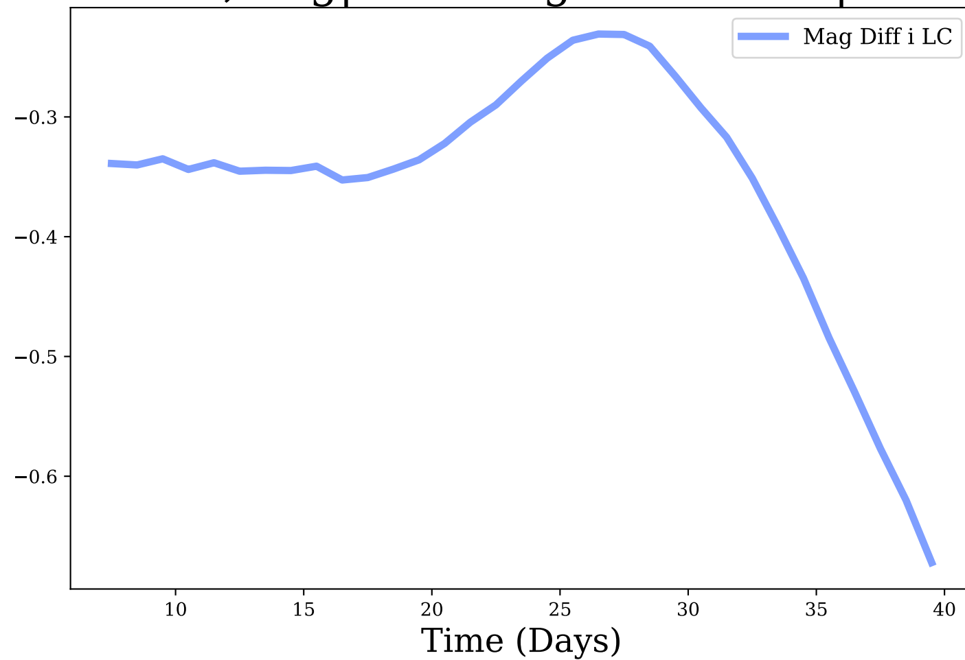
i-band, Avg|Max Mag Diff: -0.36 | 0.67
