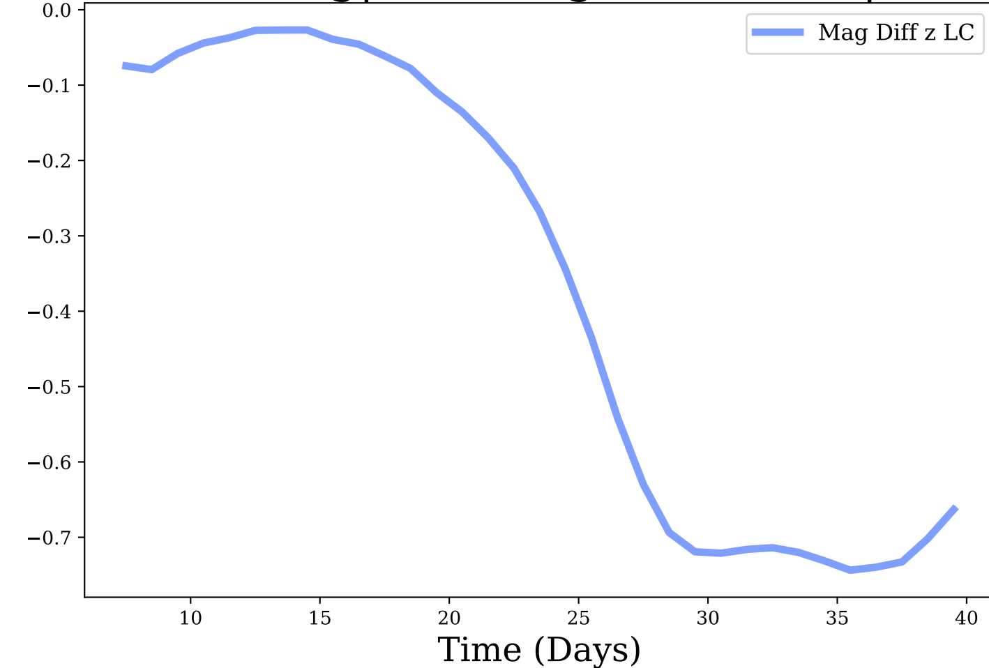
z-band, Avg|Max Mag Diff: -0.36 | 0.74
