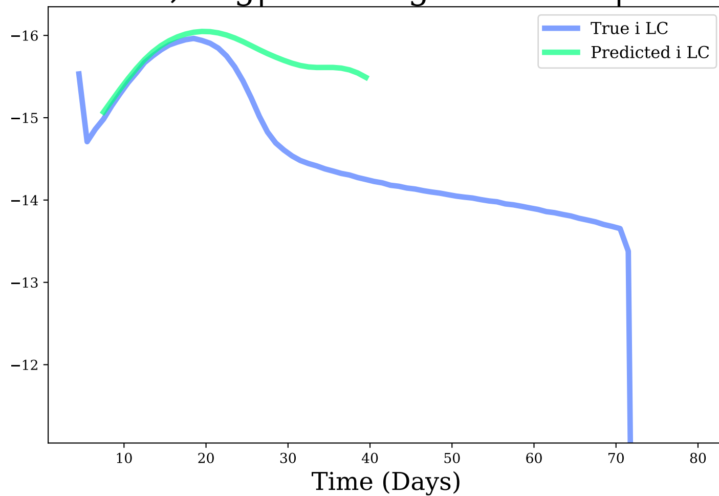
i-band, Avg|Max Mag Diff: 0.57 | 1.28
