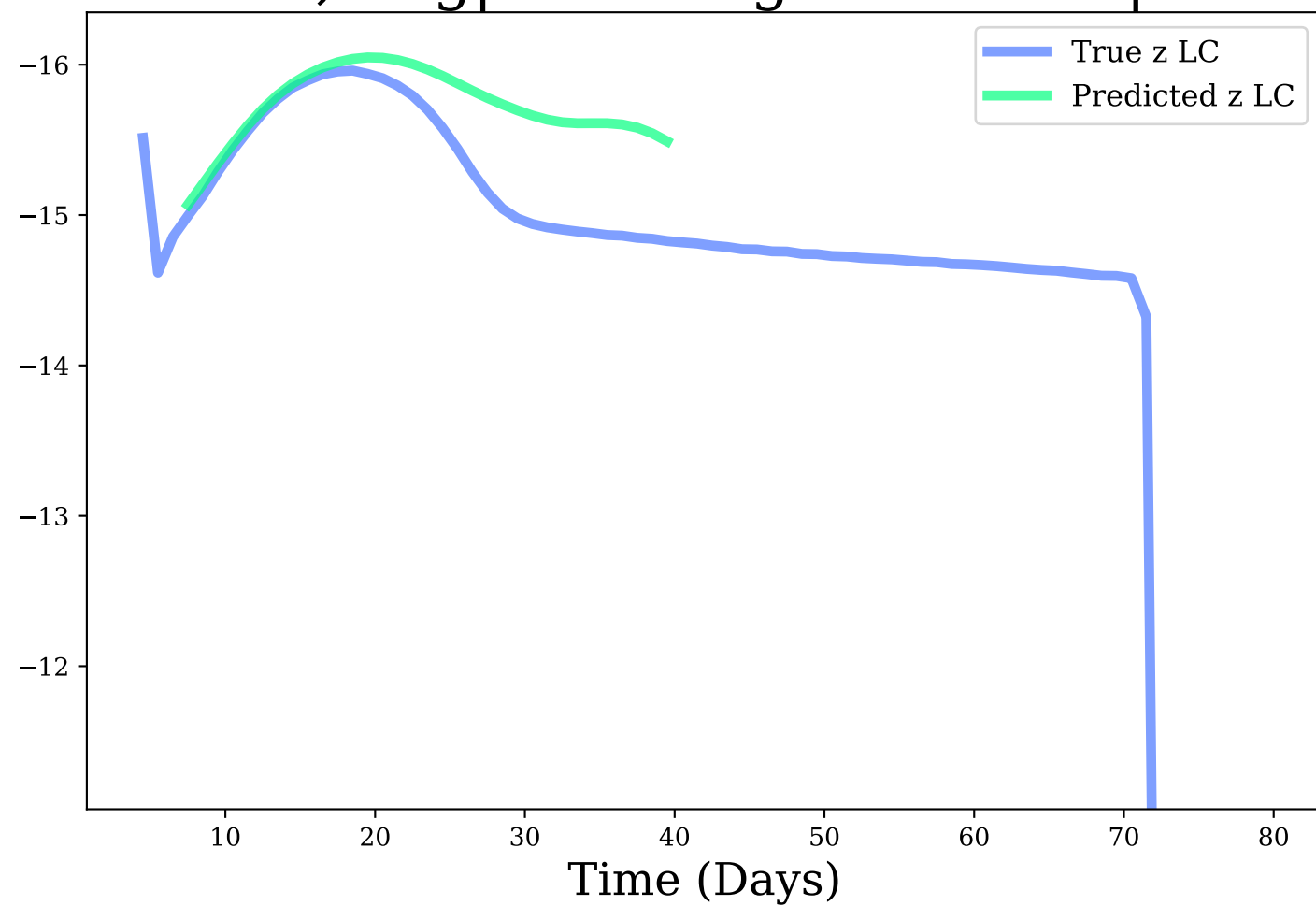
z-band, Avg|Max Mag Diff: 0.36 | 0.74
