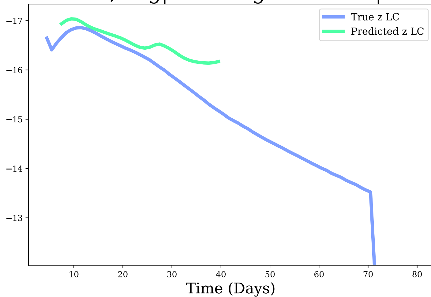
z-band, Avg|Max Mag Diff: 0.36 | 1.0
