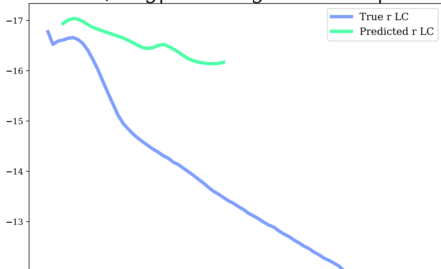
z-band, Avg|Max Mag Diff: 0.36 | 1.0
