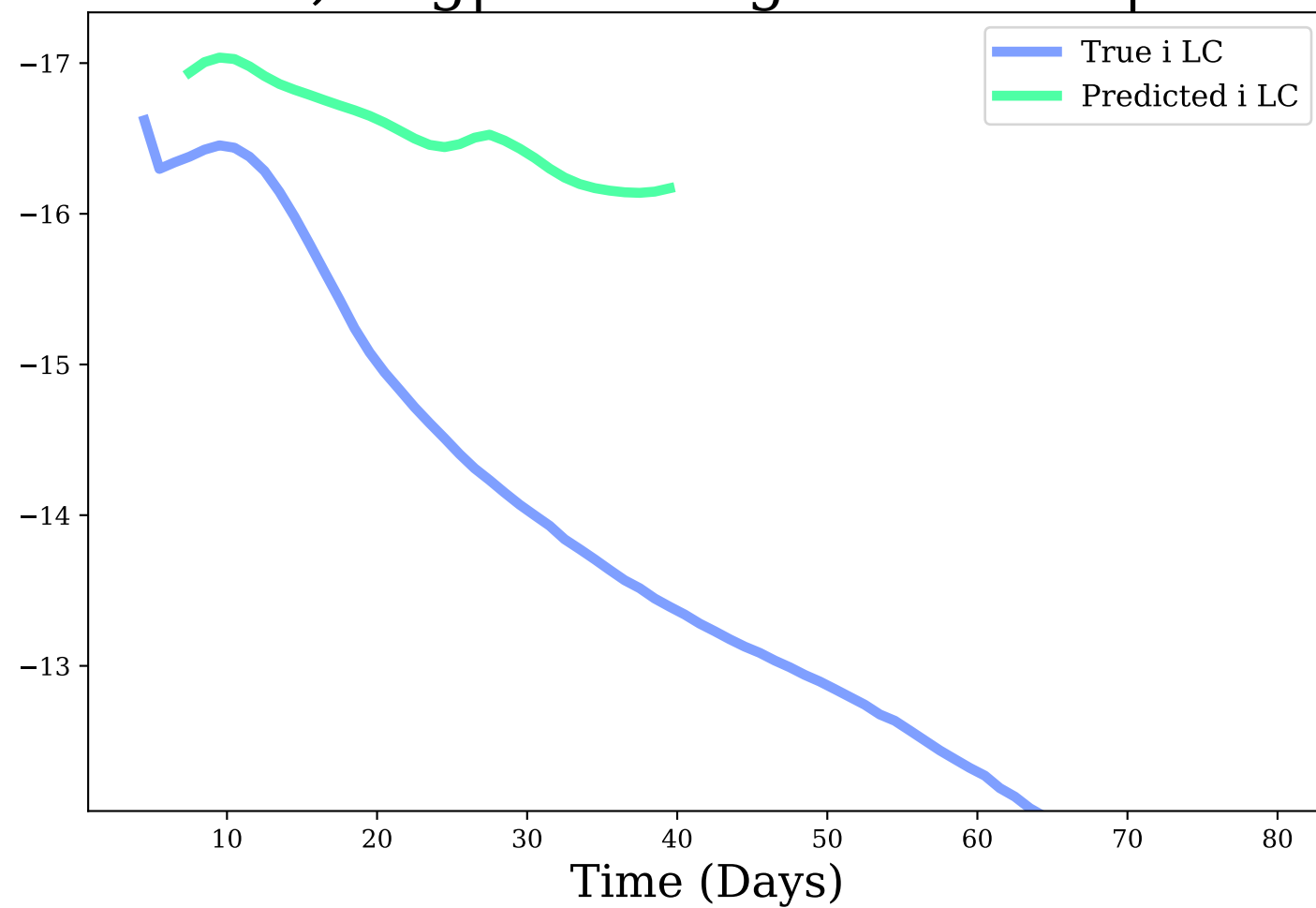
i-band, Avg|Max Mag Diff: 1.73 | 2.78
